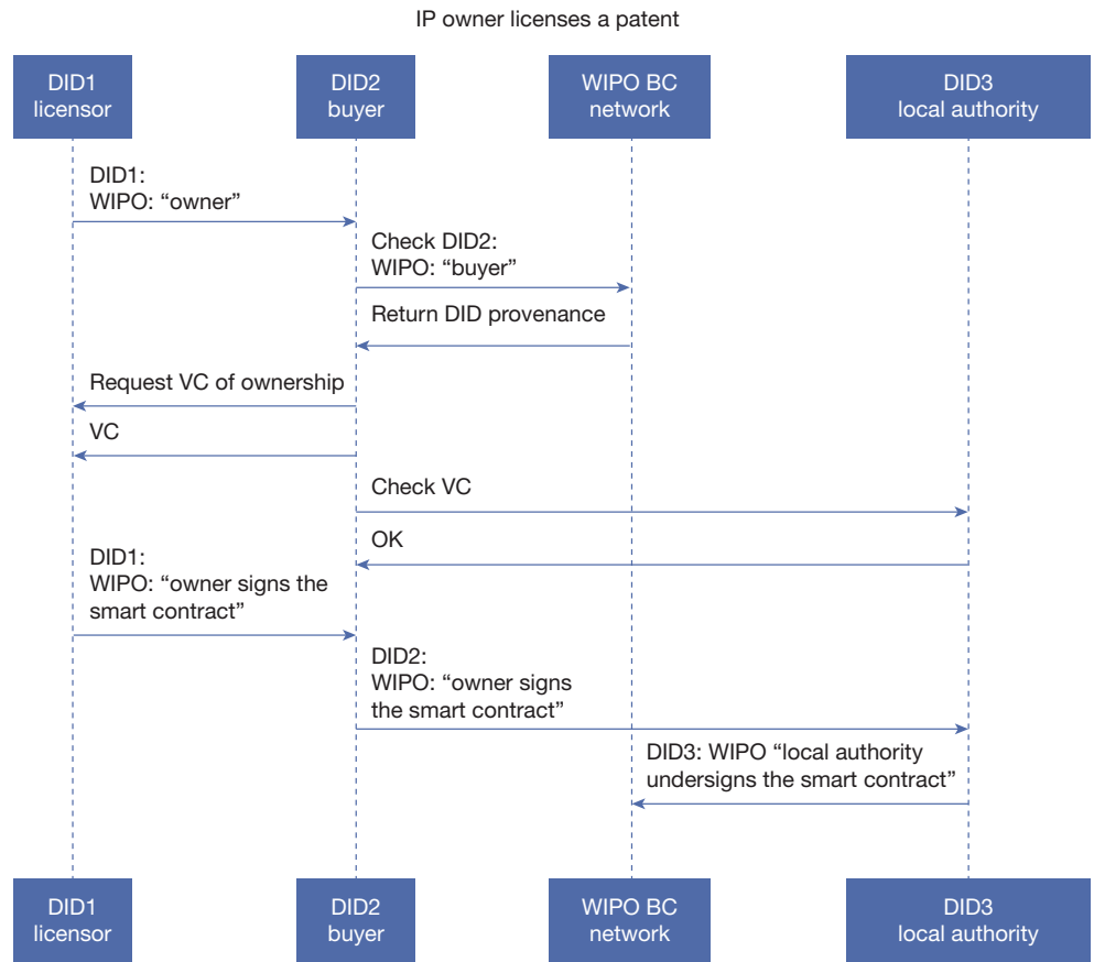
Figure 33. IP owner licenses a patent
