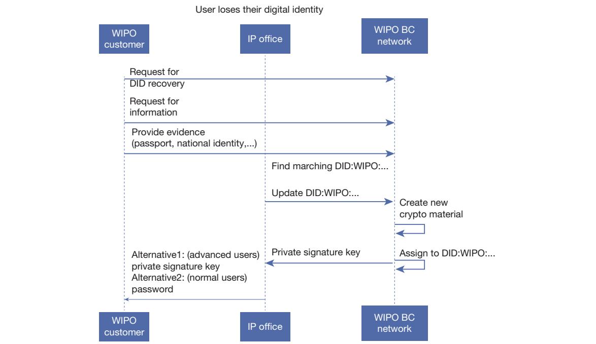
Figure 29. User loses their digital identity
