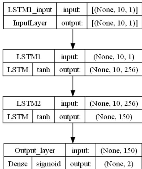
Figure 9: LSTM Model architecture for sequence-based IP-level detection.
