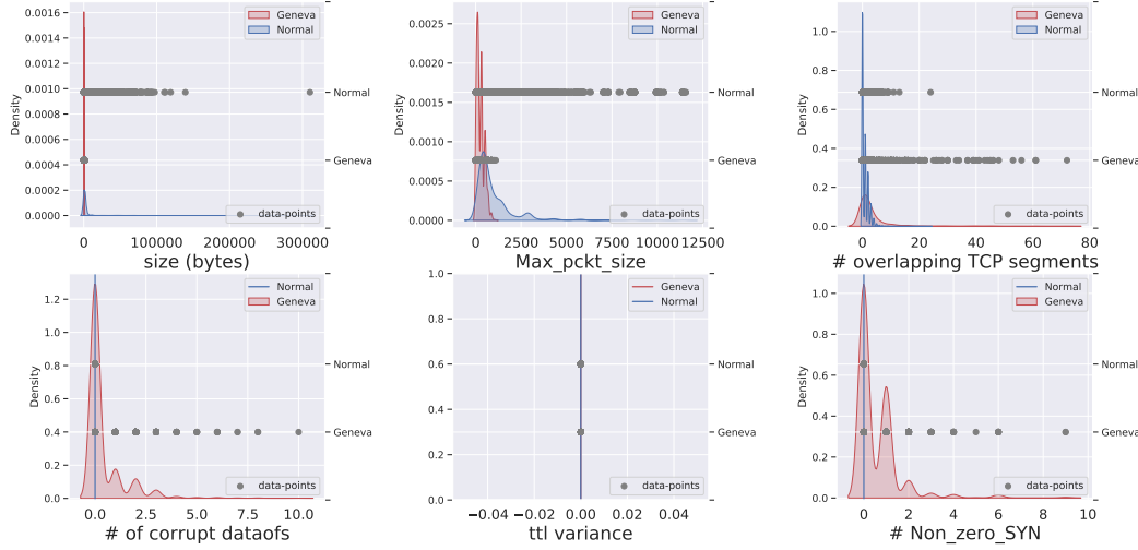
Figure 1: Geneva training feature analysis. Scatter plots show data-points of Geneva vs. normal traffic. Curves show data distribution density of each traffic type.
