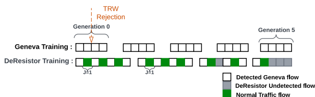
Figure 4: DeResistor System Overview. s : a manipulation strategy, P(s) : Probability that s is an evasion strategy.
