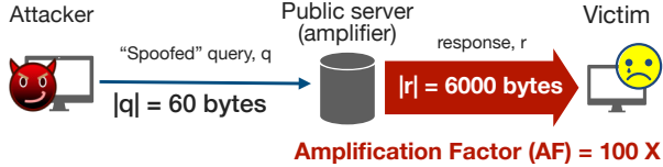
Figure 1: Primer on amplification attack and amplification factor (AF)
