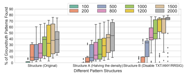
Figure 18: Validating the choice of total budget ( B_{\text{total}} )
