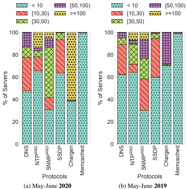
Figure 10: Summary across servers and protocols (from 2019 and 2020 runs)
