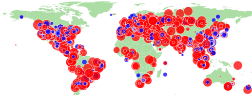
Figure 11: Visualizing the DNS residual risk when known patterns (EDNS:0 and record type:ANY |TXT) are blocked. The size of the circle \propto the max AF of each server. Red circles denote when the delta is \geq 20\% .
