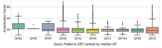
(a) Rank based on median AF
