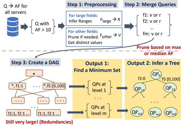
Figure 14: Steps to obtain query patterns to shed light on the patterns of amplification
