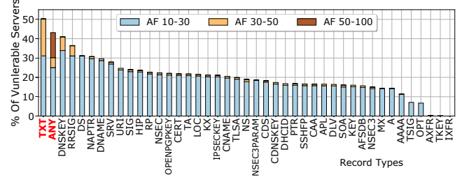
Figure 13: The variability of field values (for a specific field, record type) that contribute to high amplification. Apart from known ones (record type:ANY, TXT), many other record type values can lead to large AF.
