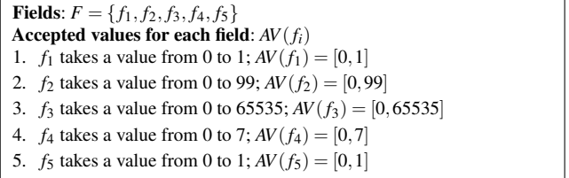
Figure 4: Simplified protocol definition to highlight challenges of uncovering amplification queries
