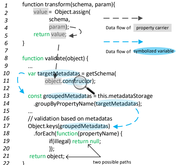
Figure 4: Illustrating the workflow of LYNX with a code snippet from our running example in §3.2 (Code is simplified for demonstration purpose).
