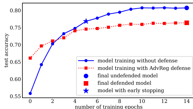
Figure 2: Test accuracy at different training epochs for Purchase100 classifiers without defense and with adversarial regularization defense [31]. We should compare the final defended model to the model with early stopping.
