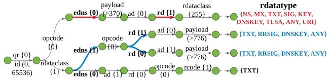
Figure 16: Tree showing how the query patterns change across levels. An edge means a field value transitioned from a wildcard (*) in level L to a concrete value or range in the next level, L + 1 .
