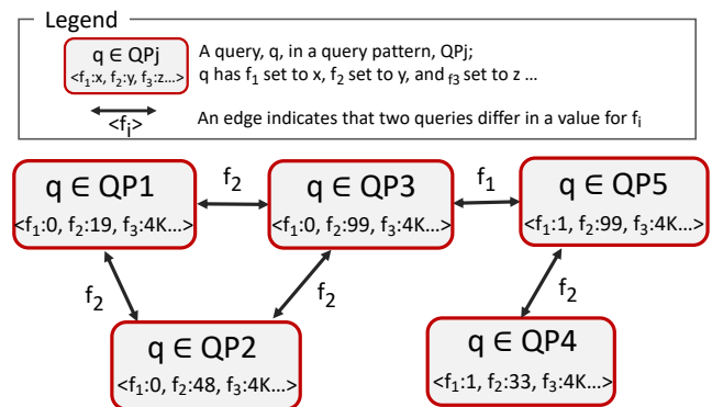
Figure 7: Viewing the query space as a logical graph (for the abstract protocol shown in Figure 5)
