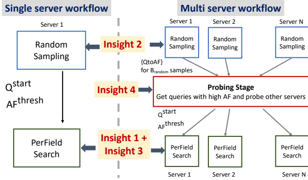
Figure 8: AmpMap Workflow
