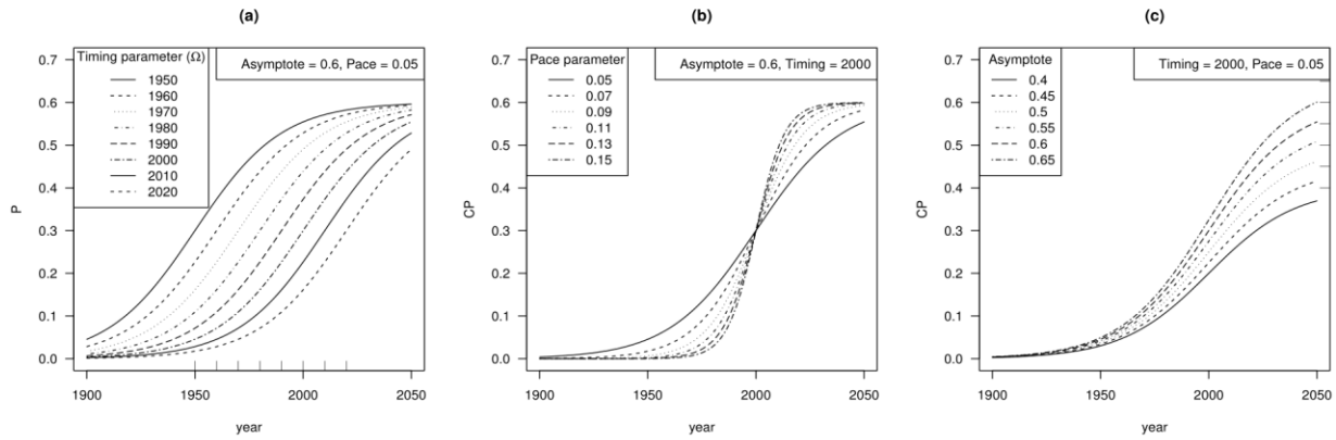
Figure 5 Stylized logistic curves under different values of each of the three logistic parameters: (a) timing; (b) pace; (c) asymptote. In each panel, one parameter is changed and the other two are held constant at the values specified.
