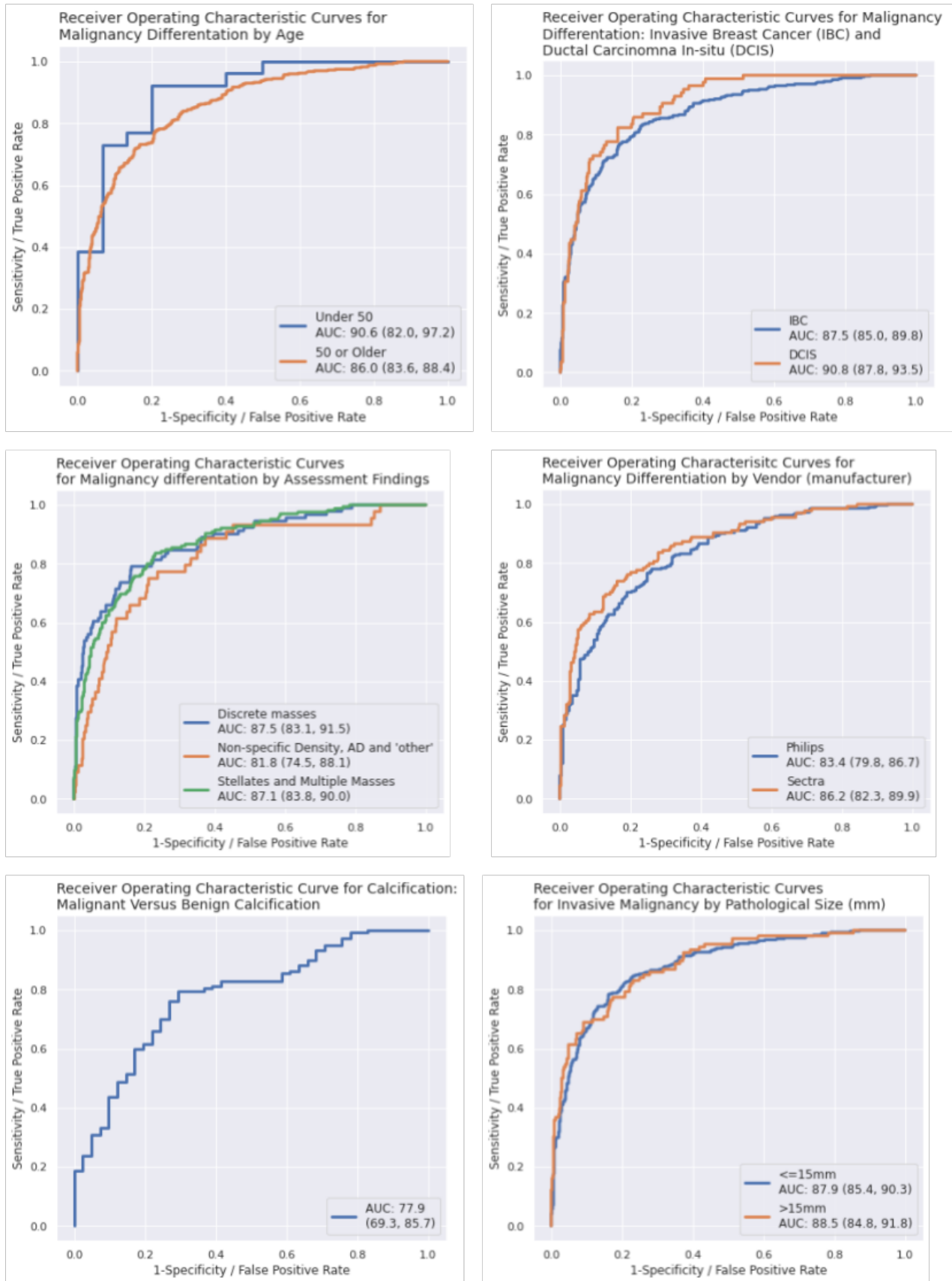
Fig. S1. Secondary results by client and radiological strata for NYU2 retrained with transfer learning.
