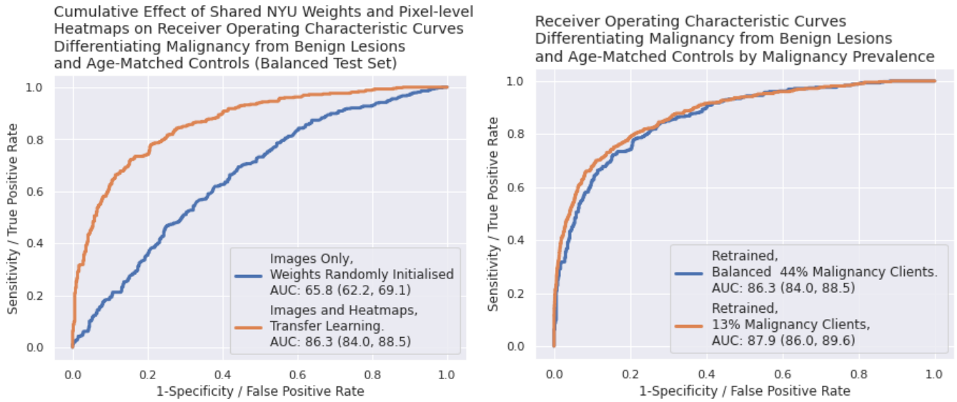
Fig. S2. Left: cumulative effect of NYU heatmaps and weights. Right: AUROC by malignancy incidence
