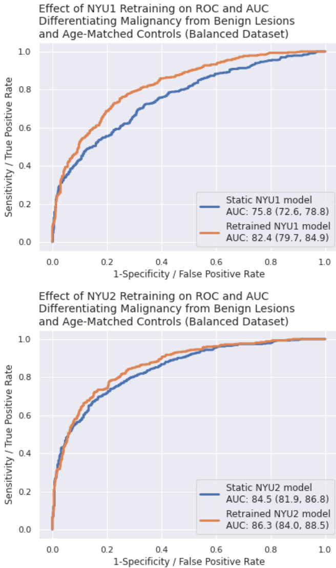
Fig. 3. Top: Effect of retraining image-only (NYU1) model. Bottom: Effect of retraining image and heatmaps (NYU2) model.
