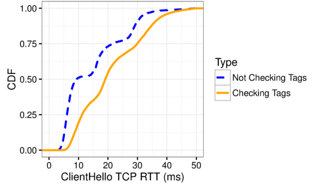
Fig. 5. CDFs comparing the TCP round trip time (RTT) for TLS ClientHello packets with tag checking on and off.
