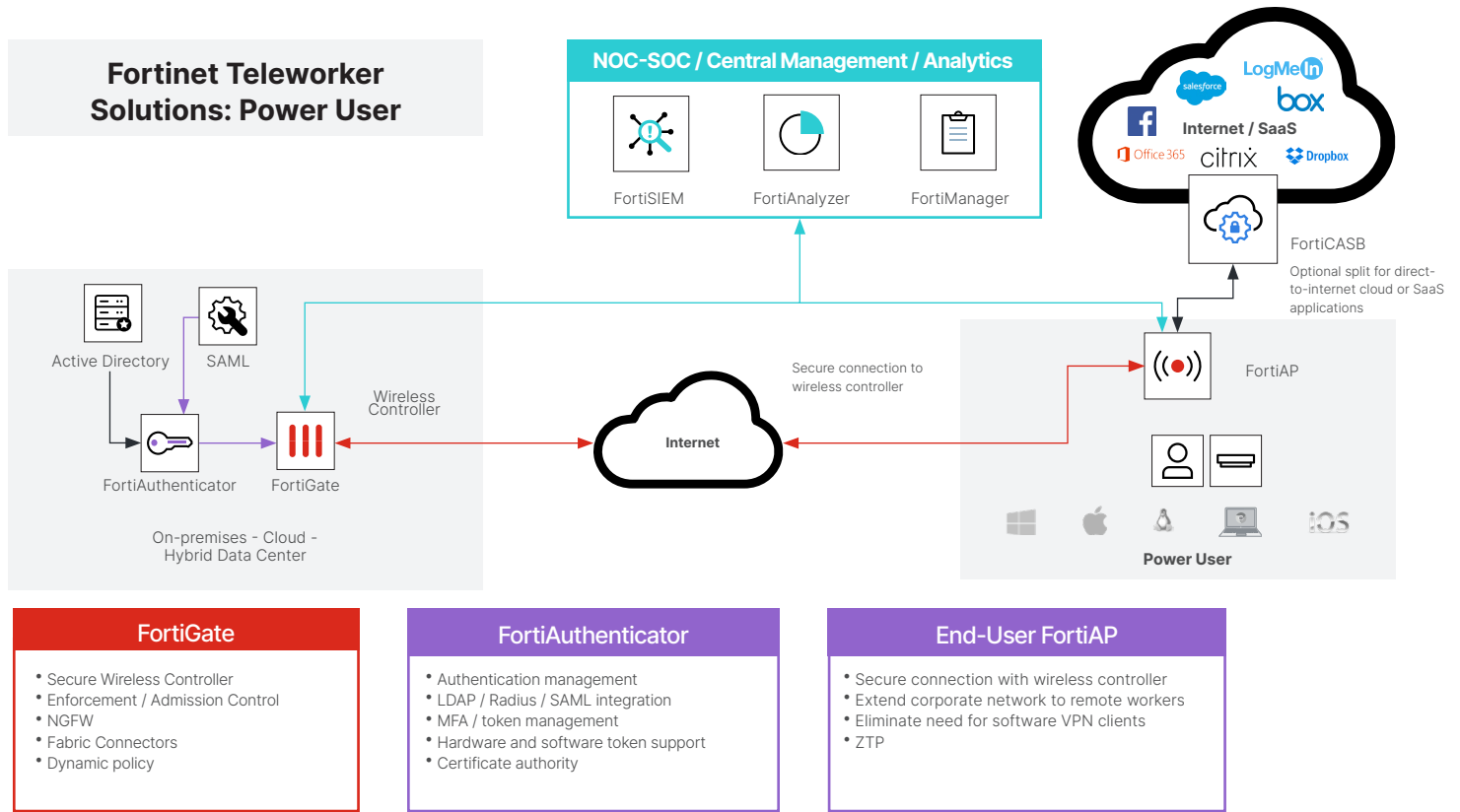
Figure 2: Notional Fortinet solution deployment for power user.
