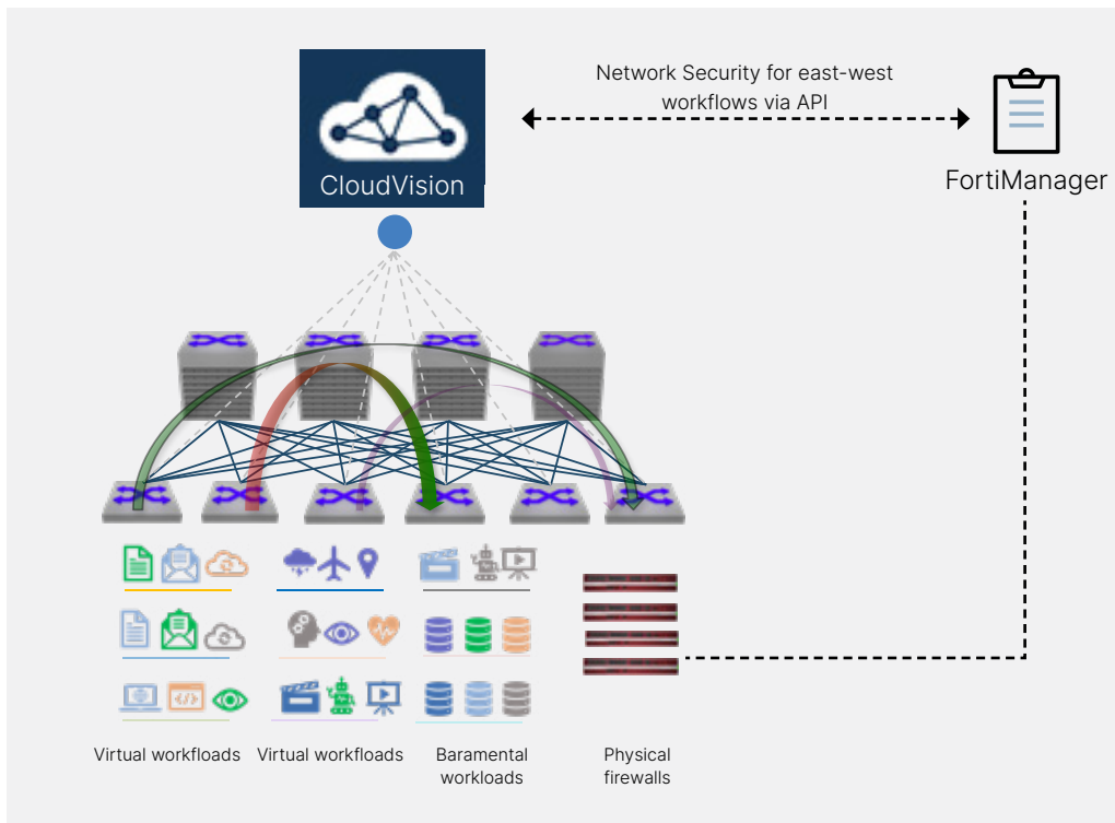
Figure 1: Fortinet FortiGate and Arista MSS-FW joint solution.
