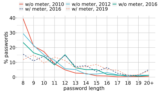
Figure 8: Length distribution for 1c8 passwords collected in studies over time.
