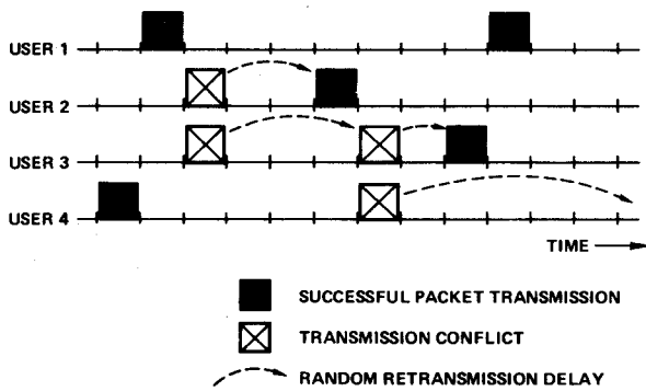
Fig. 1. Slotted ALOHA random access.
