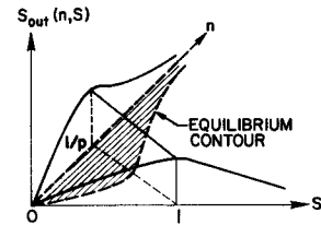
Fig. 3. Throughput surface above the (n, S) plane.
