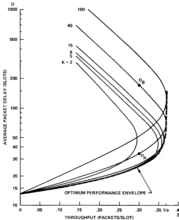
Fig. 2. Equilibrium throughput-delay tradeoff.
