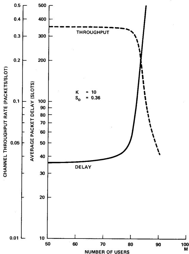
Fig. 8. Channel performance versus M at K = 10 and S_o = 0.36 .
