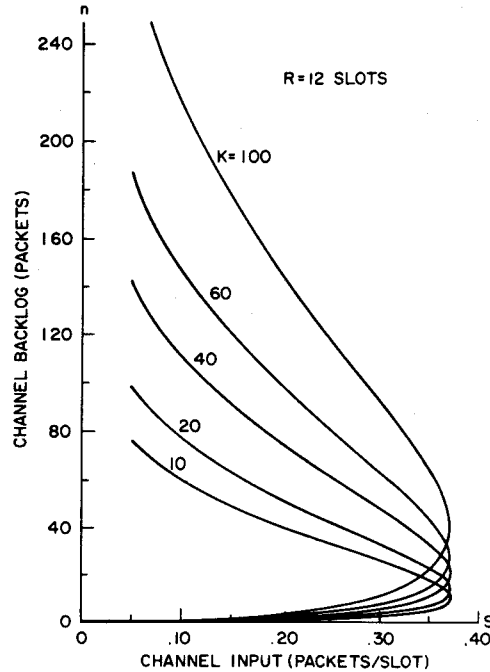
Fig. 4. Equilibrium contours in the (n, S) plane.
