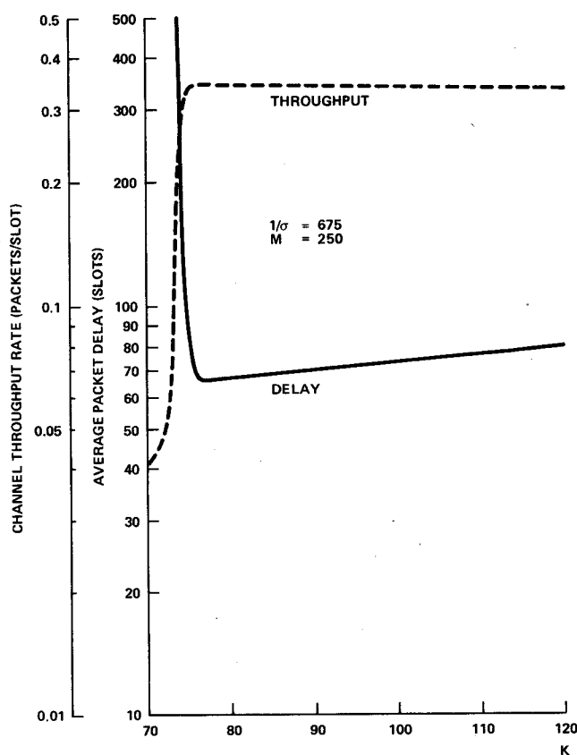
Fig. 11. Channel performance versus K at M = 250 and 1/\sigma = 675 .
