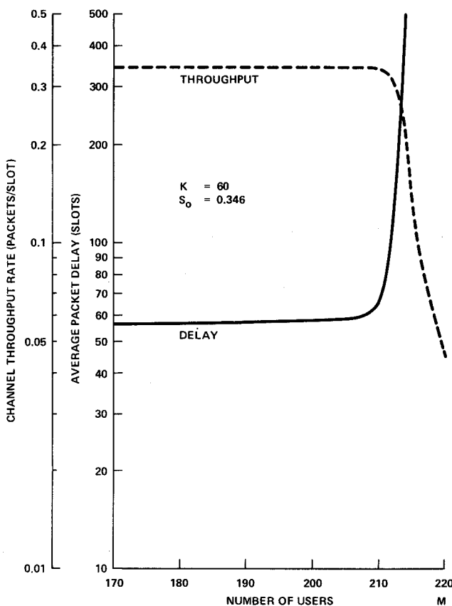
Fig. 9. Channel performance versus M at K = 60 and S_o = 0.346 .
