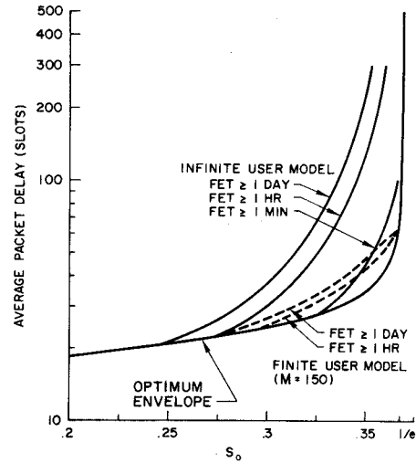
Fig. 15. Stability-throughput-delay tradeoff.
