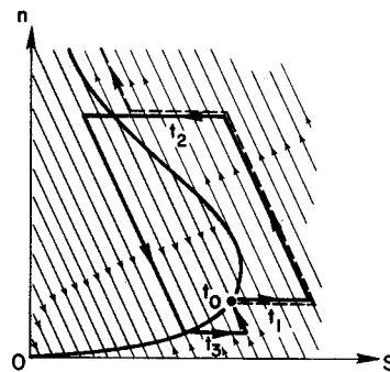
Fig. 6. Fluid approximation trajectories.
