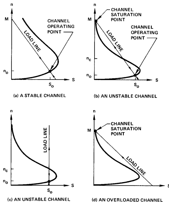
Fig. 7. Stable and unstable channels.
