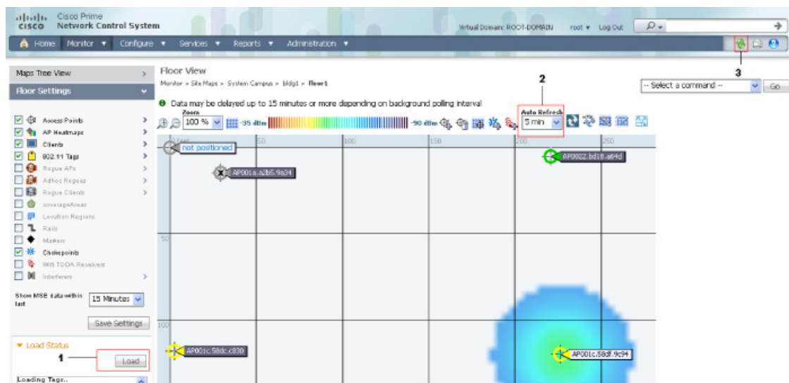
Figure 6-45 Refresh Options
