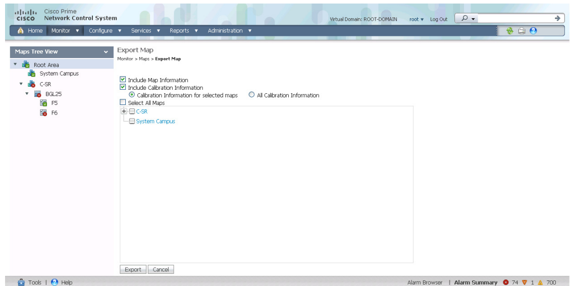
Figure 6-9 Export Map
