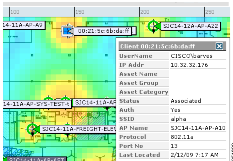
Figure 6-51 Client Details
