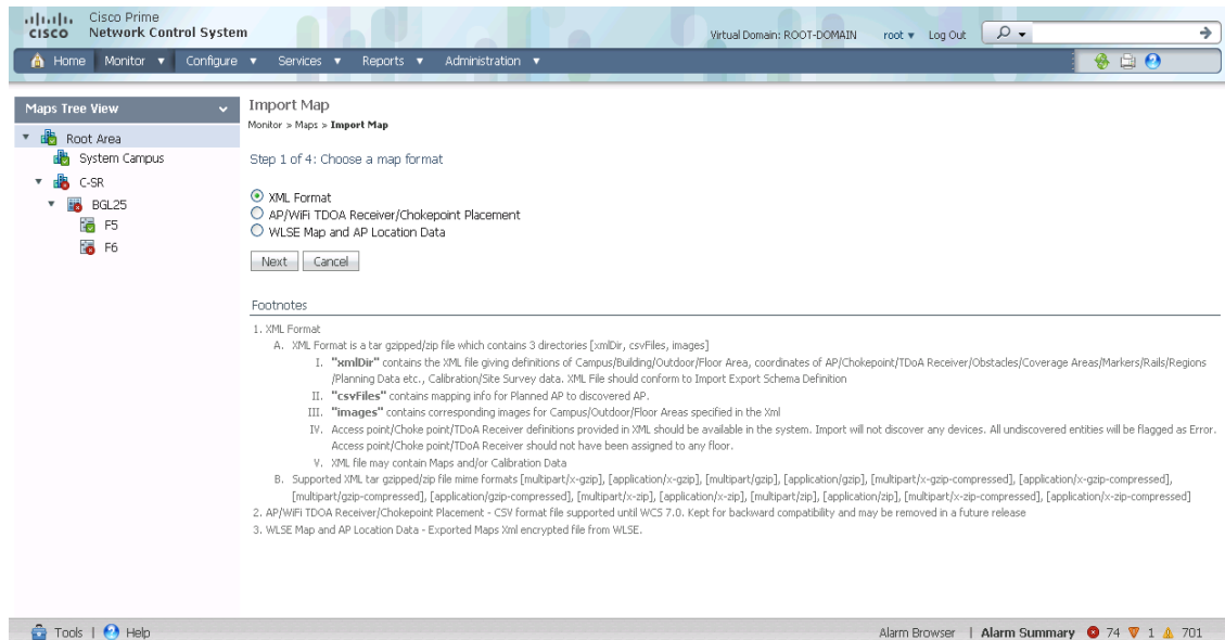
Figure 6-10 Import Map
