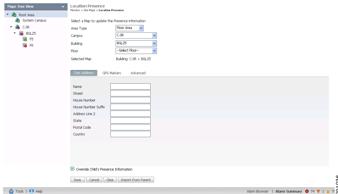
Figure 6-12 Location Presence
