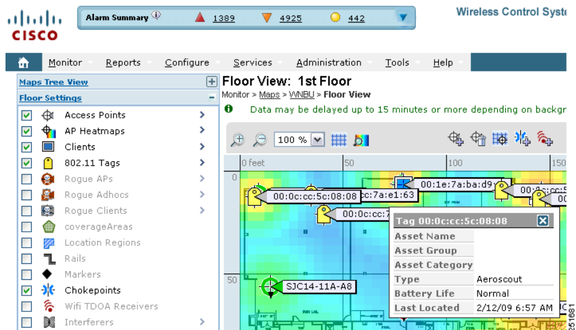
Figure 6-52 Tag Details
