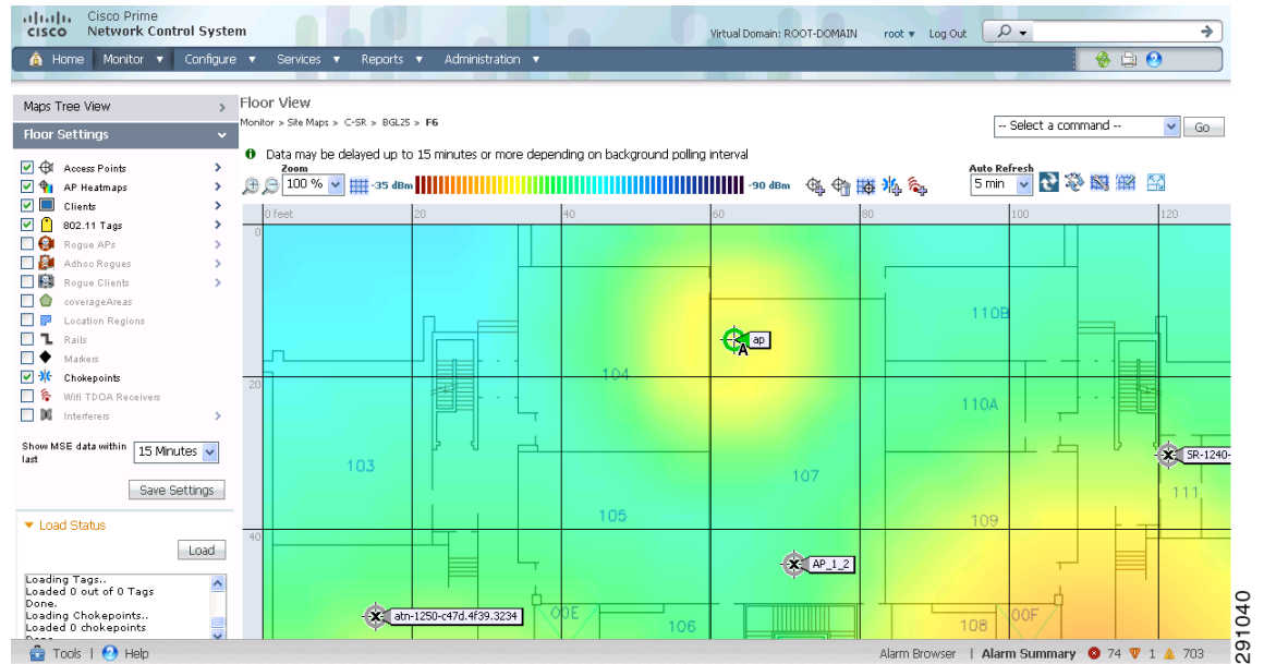
Figure 6-19 Floor View
