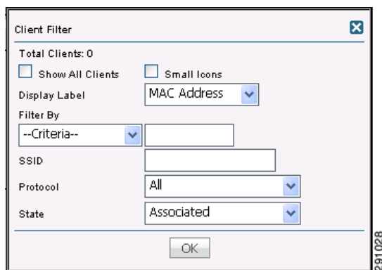
Figure 6-26 Client Filter
