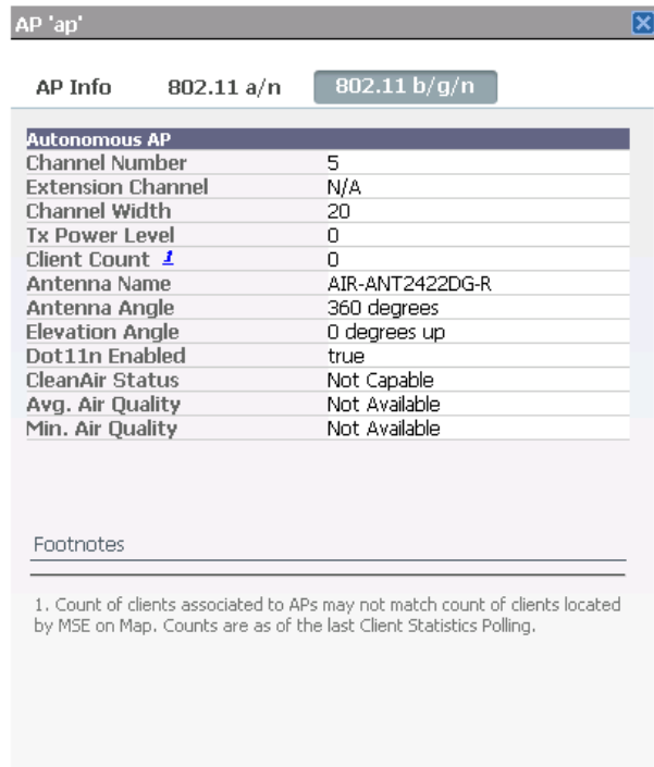
Figure 6-50 802.11 Tabs
