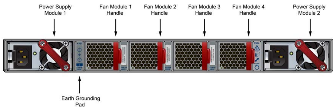
Figure D-1: Rear Panel for Models with Management Ports in the Front
