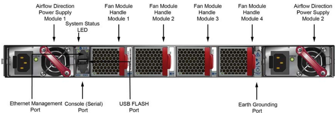
Figure D-2: Rear Panel for Models with Management Ports in the Rear
