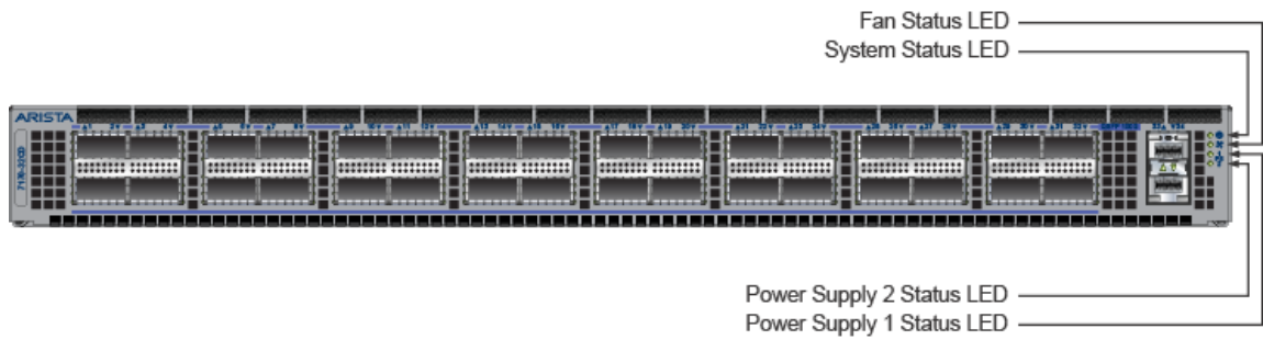
Figure C-5: DCS-7170-32CD
