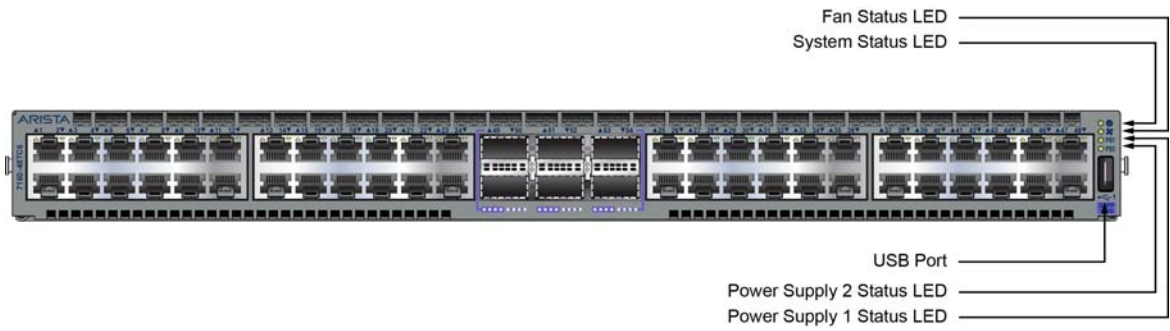
Figure C-3: DCS-7160-48TC6
