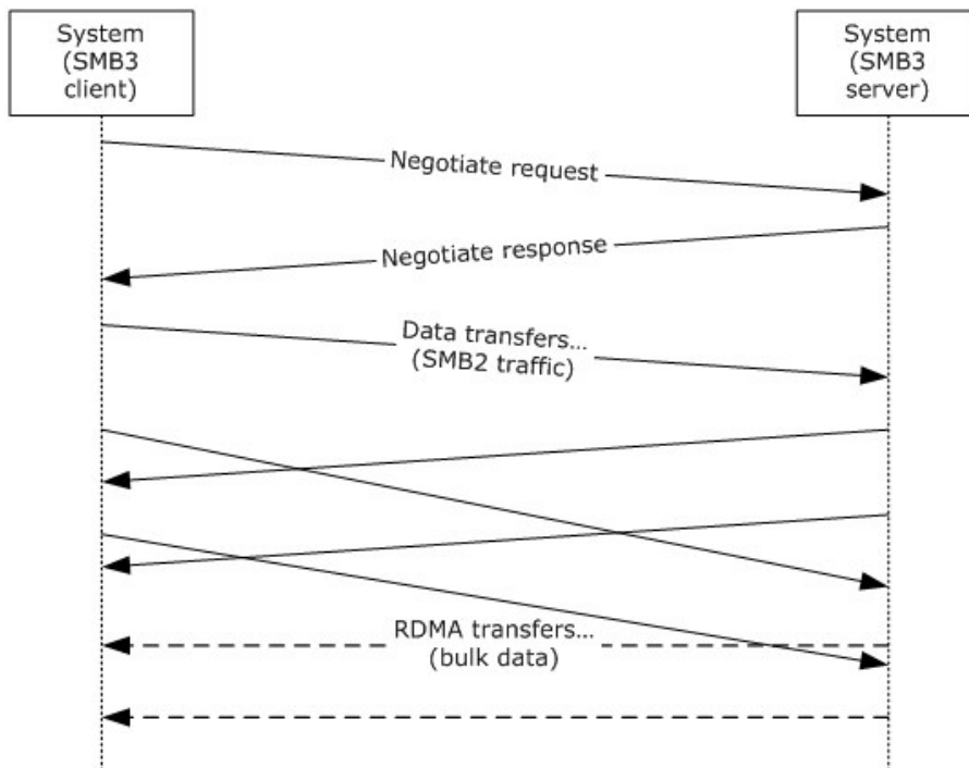
Figure 1: Data transfer
