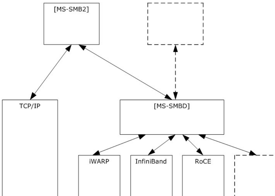
Figure 2: Protocol relationships
