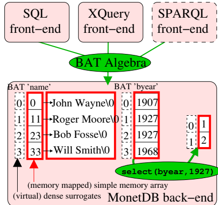
Figure 3.2: MonetDB: BAT Algebra Execution.
