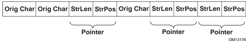
Figure 65. Block Body
