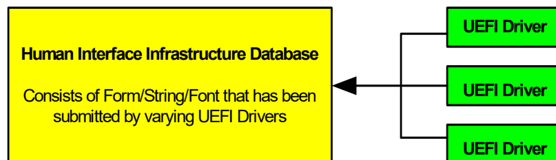
Figure 109. HII Database
