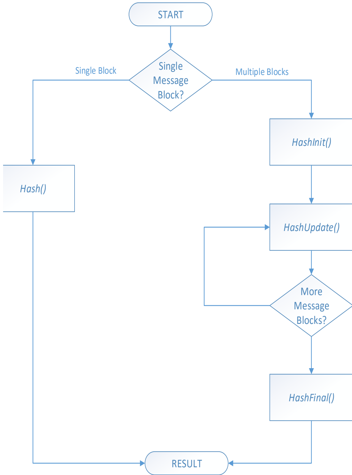
Figure 140. Hash workflow
