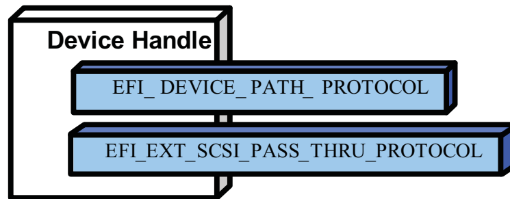
Figure 56. Device Handle for a SCSI Bus Controller
