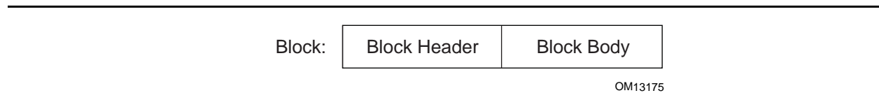
Figure 64. Block Structure
