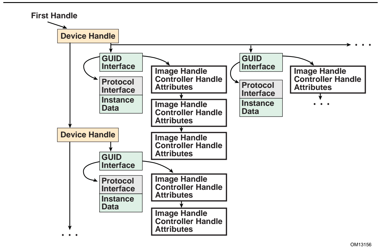
Figure 26. Handle Database
