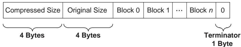
Figure 63. Compressed Data Structure
