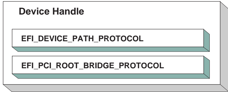
Figure 46. Device Handle for a PCI Host Bus Controller
