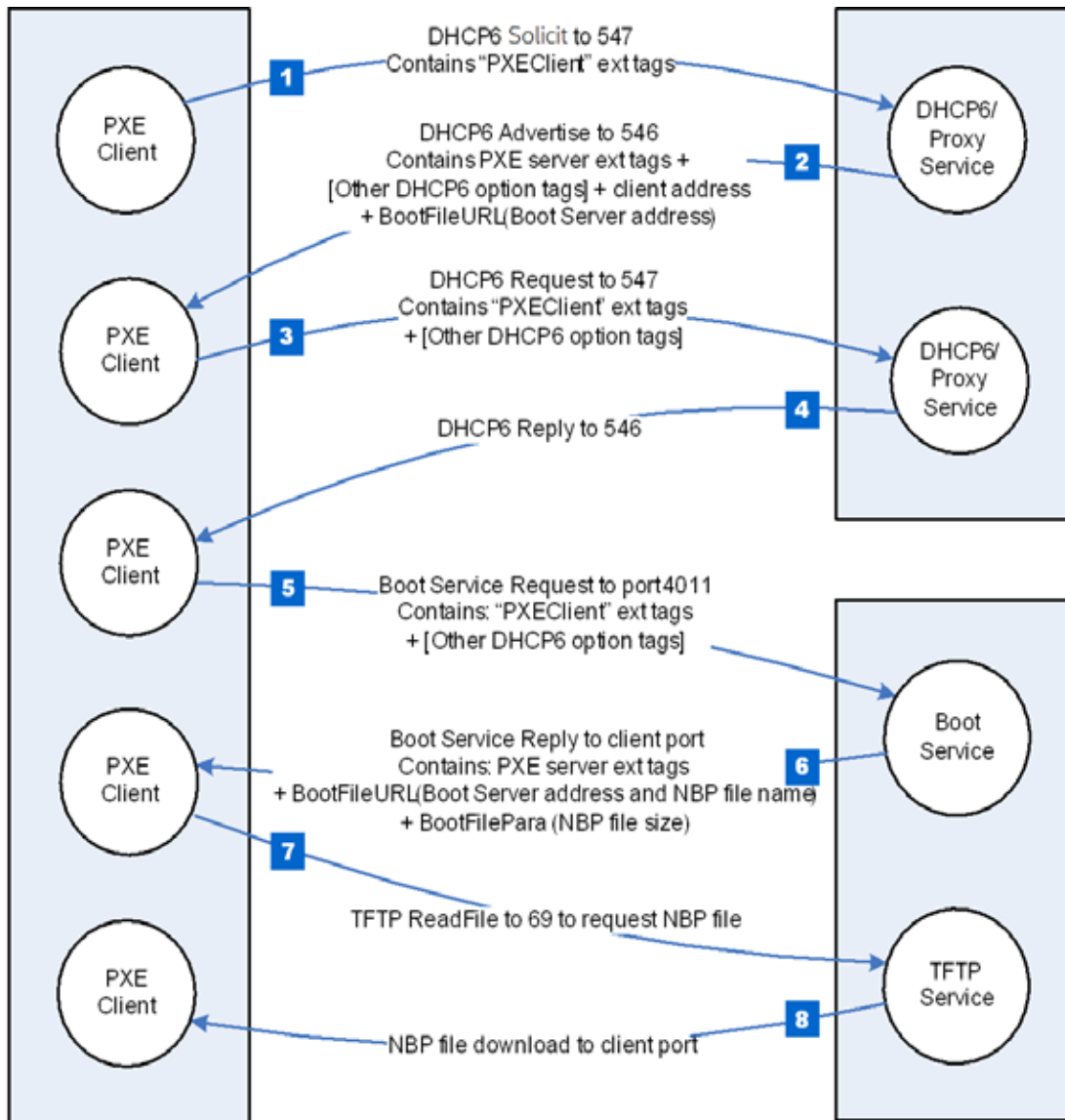
Figure 73. IPv6-based PXE boot
