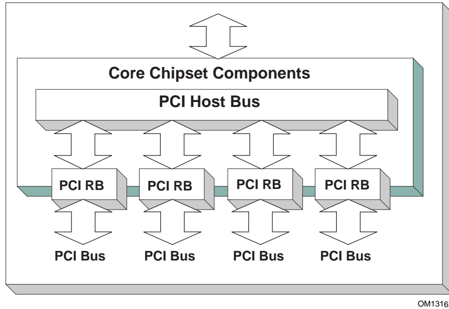
Figure 40. Server System with Four PCI Root Bridges
