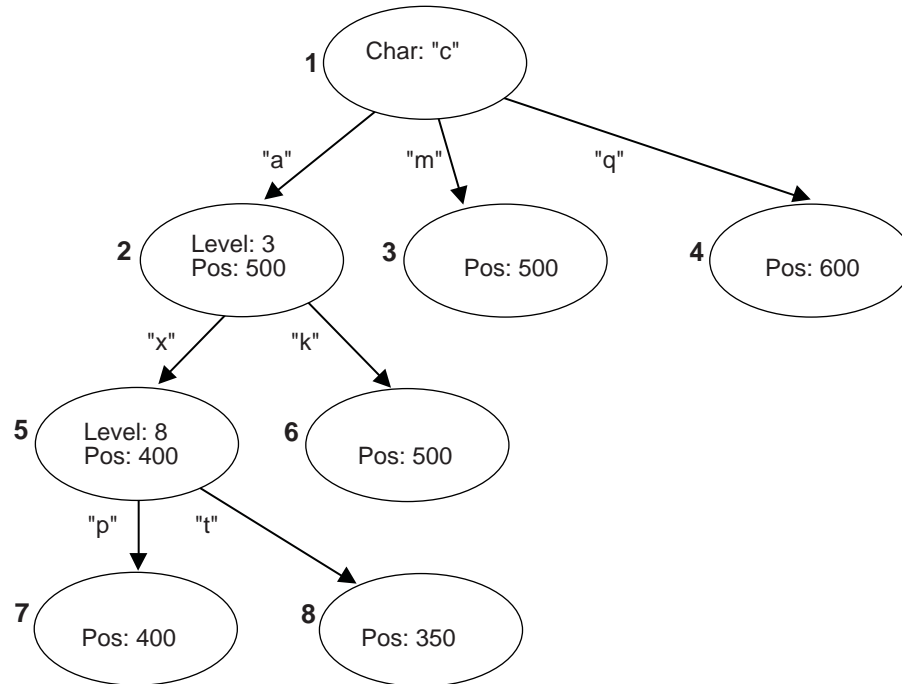
Figure 66. String Info Log Search Tree
