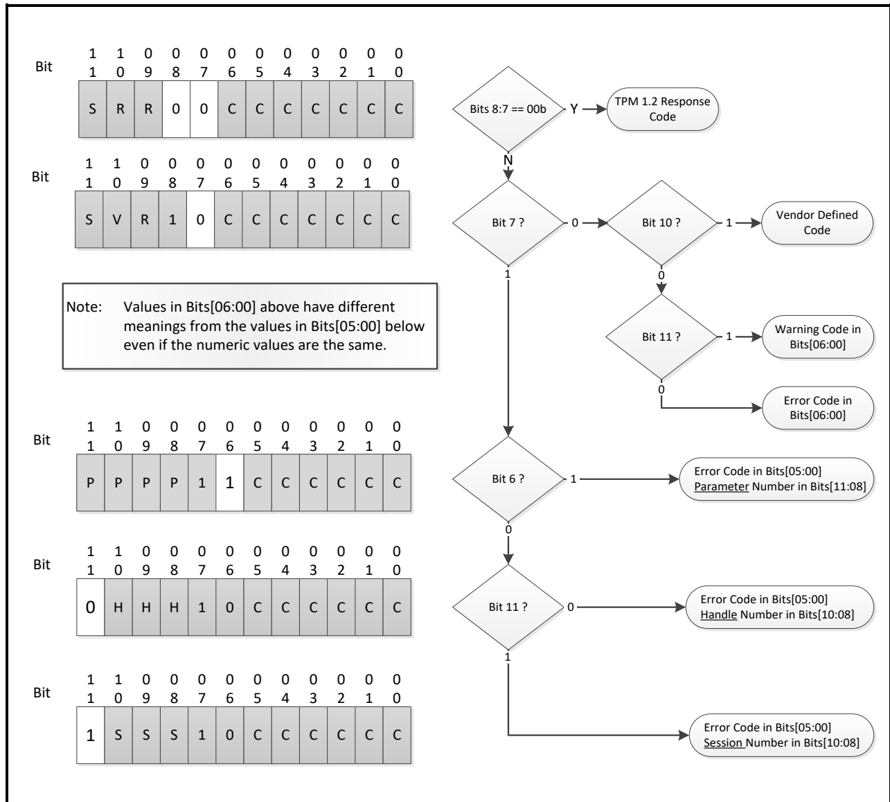
Figure 27 — Response Code Evaluation
