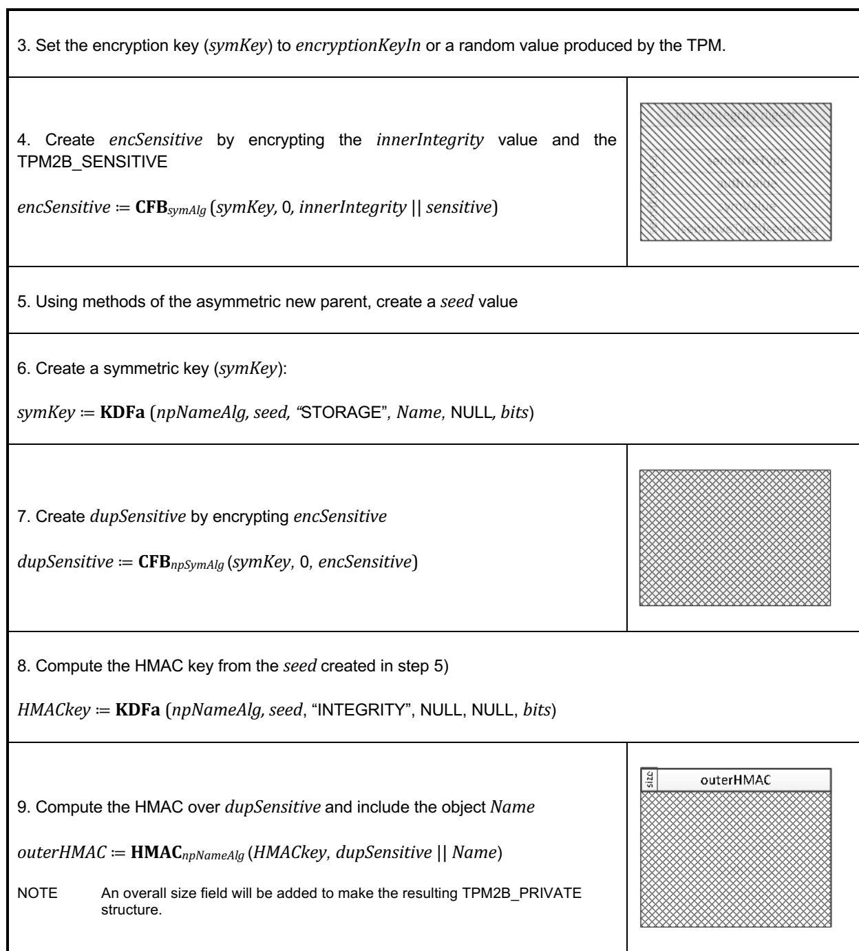
Figure 19 — Duplication Process with Inner and Outer Wrapper
