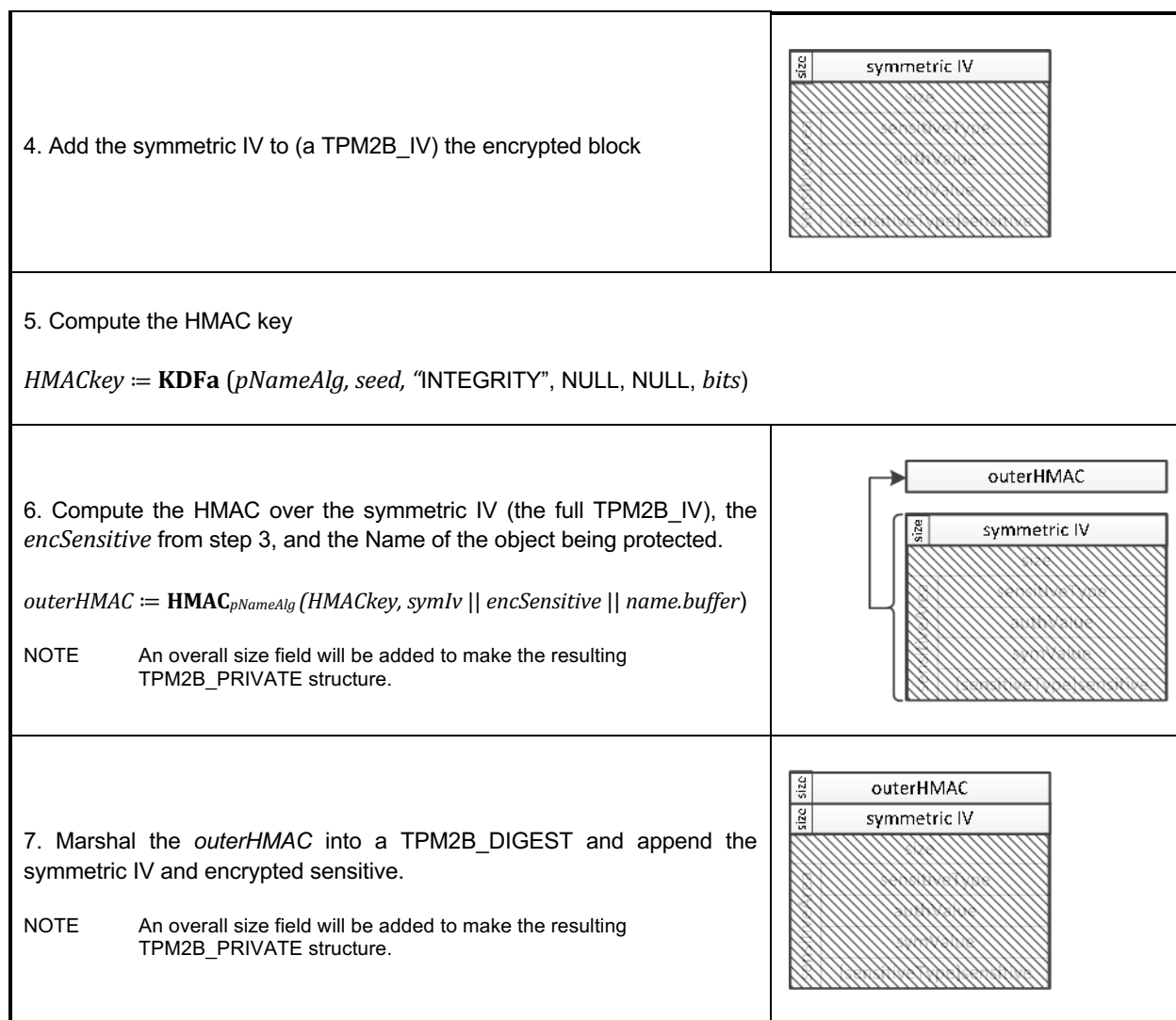
Figure 17 — Creating a Private Structure
