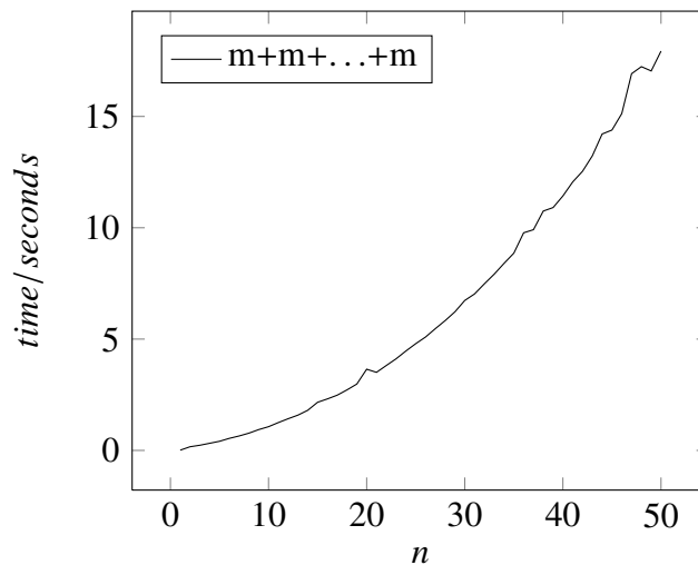
Figure 6.23: Processing time increasing with length of expression
