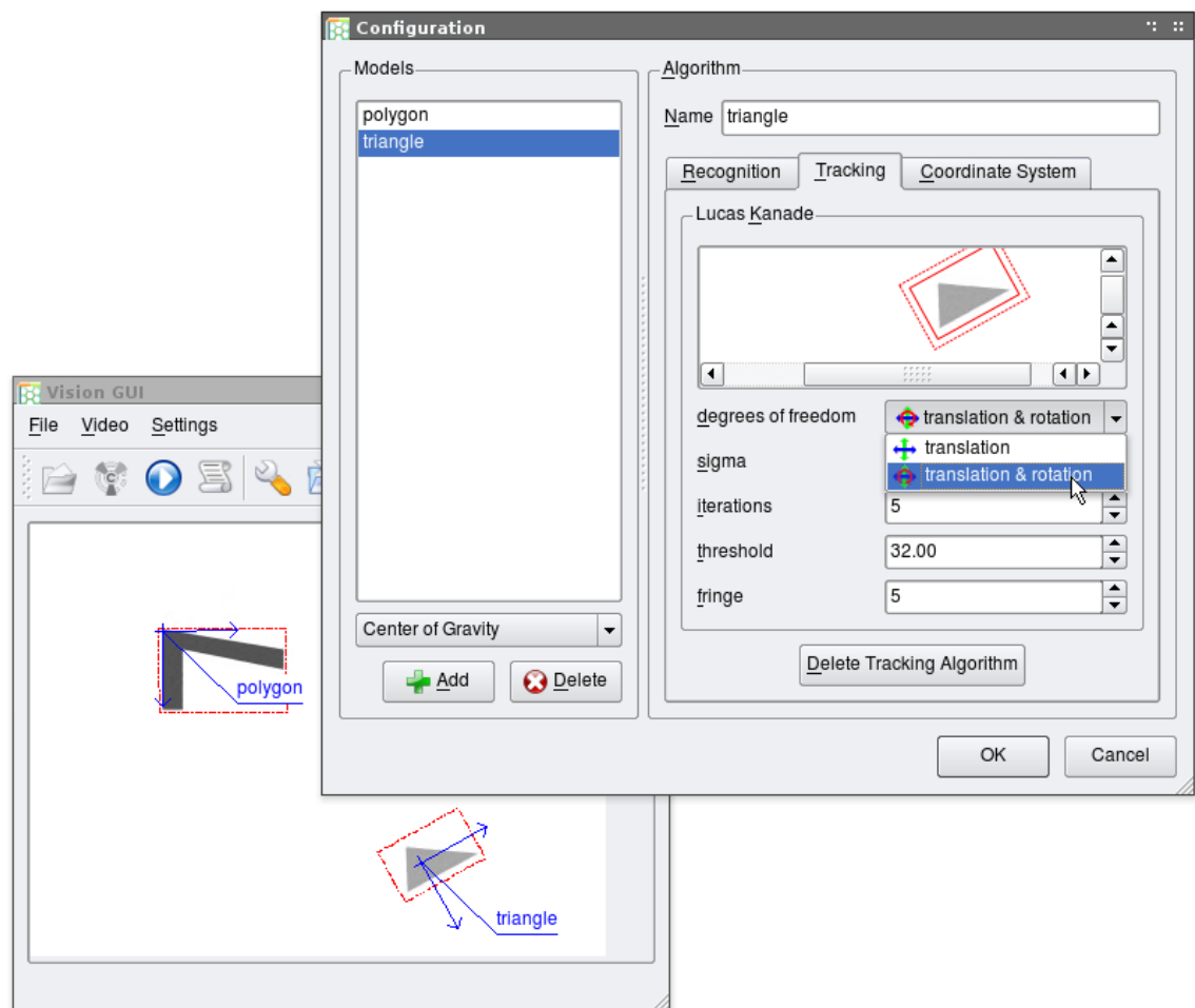
Figure 6.7: Configuration GUI
