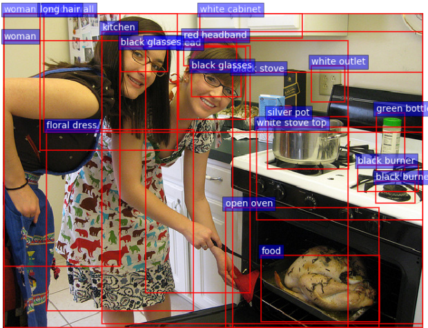
Figure 2. Example output from our Faster R-CNN bottom-up attention model. Each bounding box is labeled with an attribute class followed by an object class. Note however, that in captioning and VQA we utilize only the feature vectors – not the predicted labels.
