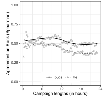
(b) Agreement on ranks between measures of bug finding and #branches after a campaign of x hours.
