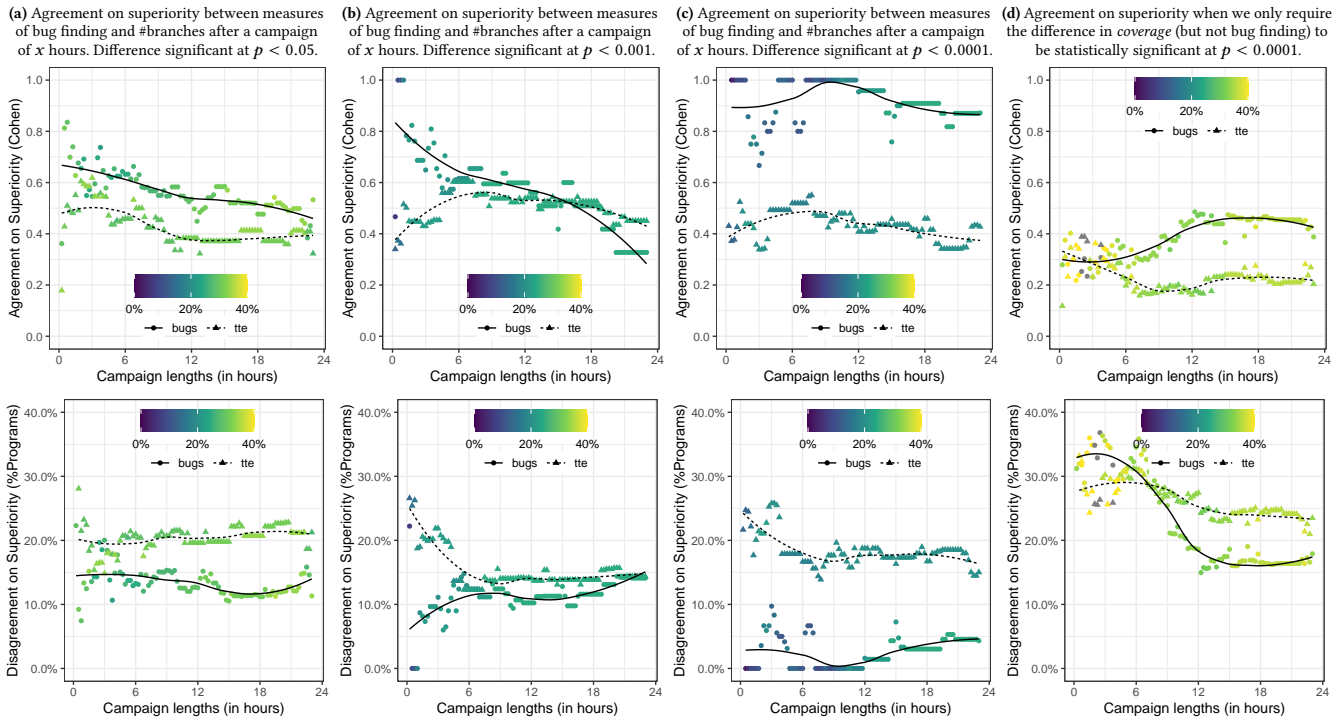
Figure 9: Agreement on superiority over campaign length. We show agreement when evaluating fuzzer performance based on branch coverage versus the number of bugs (solid line) and branch covered versus the time-to-error (dashed line). The color shows the percentage of fuzzer pairs for which the differences are statistically significant at the corresponding p -value ( p \leq \{0.05, 0.001, 0.0001\} ).
