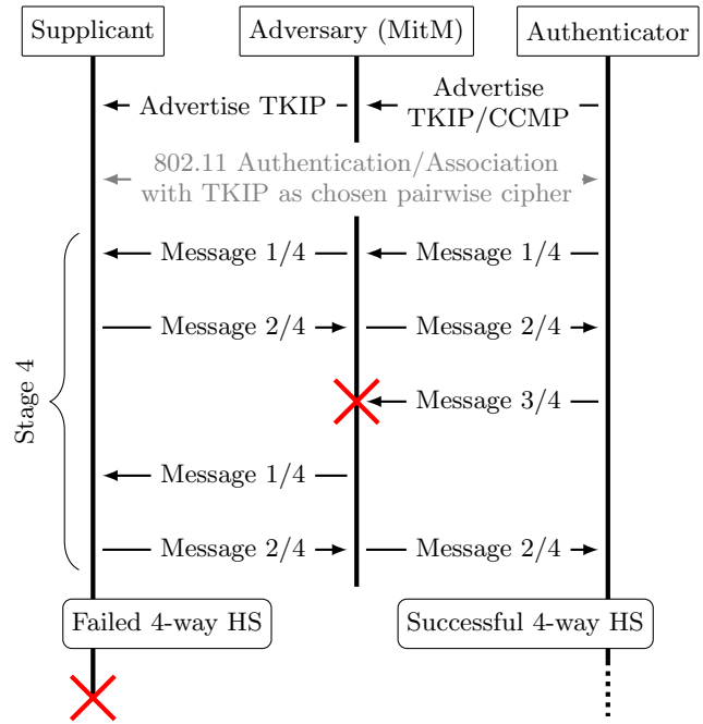
Figure 3: Downgrading a Broadcom authenticator to TKIP, when both TKIP and CCMP is enabled. The attack only works against WPA1, since Broadcom only confuses message 2 and 4 in WPA1.
