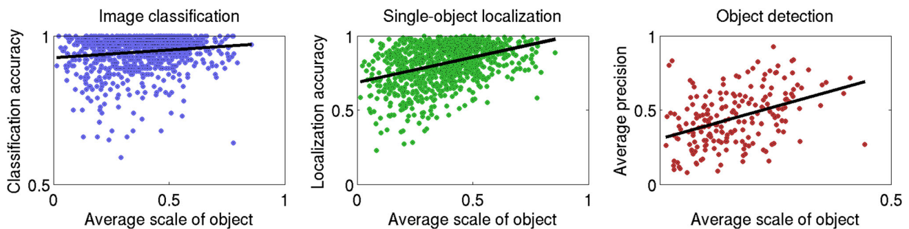
Fig. 13 Performance of the “optimistic” method as a function of object scale in the image, on each task. Each dot corresponds to one object class. Average scale (x-axis) is computed as the average fraction of the image area occupied by an instance of that object class on the ILSVRC2014 validation set. “Optimistic” performance (y-axis) corresponds to the best performance on the test set of any entry submitted
