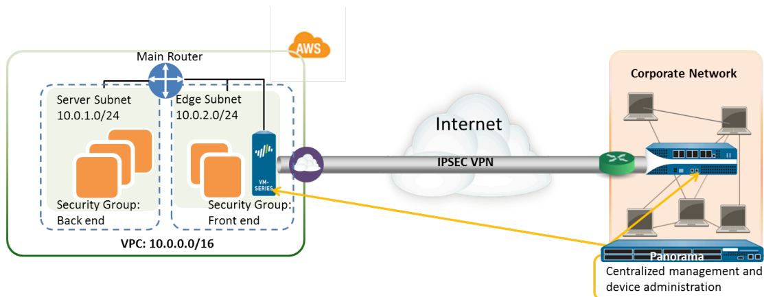
Figure 2: VM-Series for VPN Access
