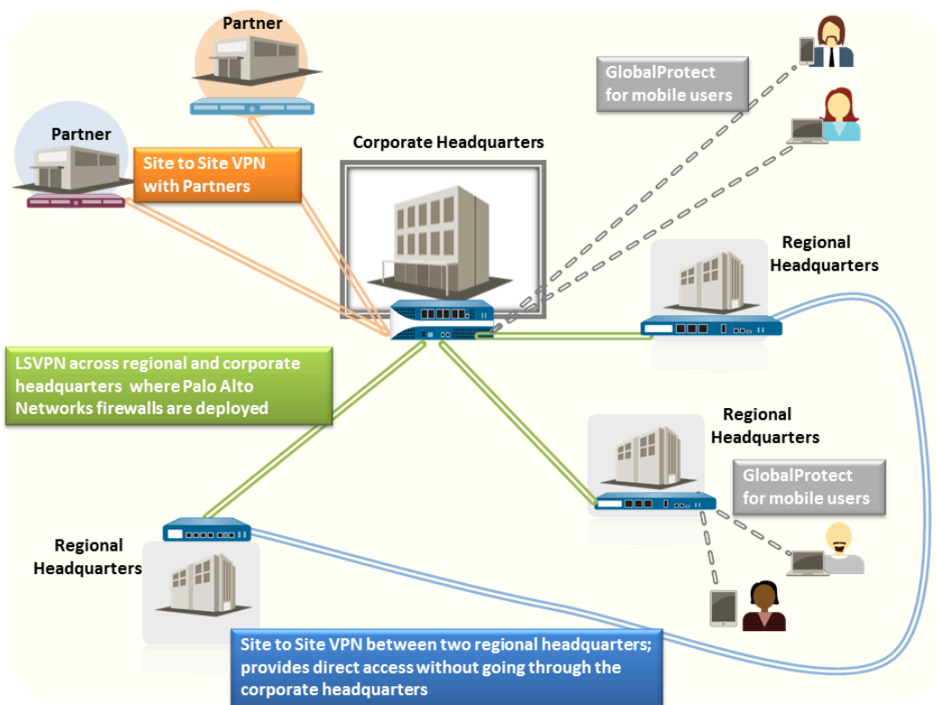
Figure 7: VPN Deployments
