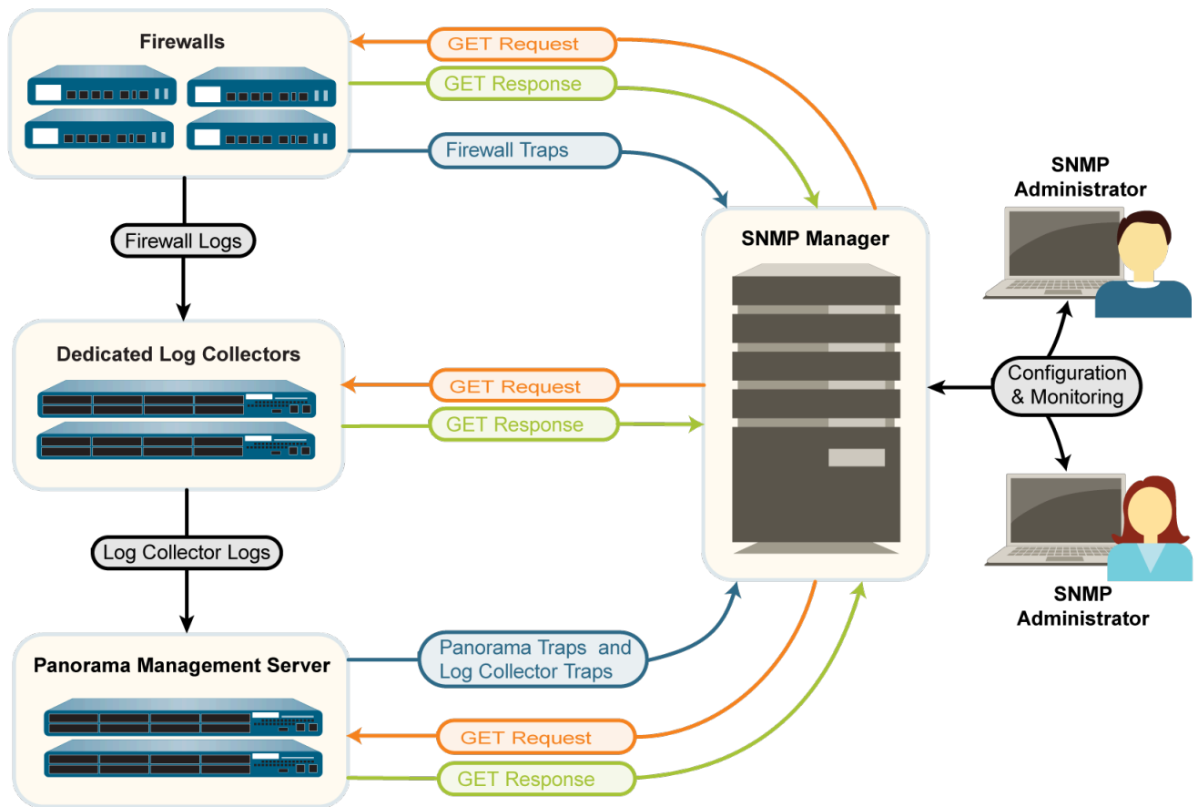
Figure 2: SNMP Implementation
