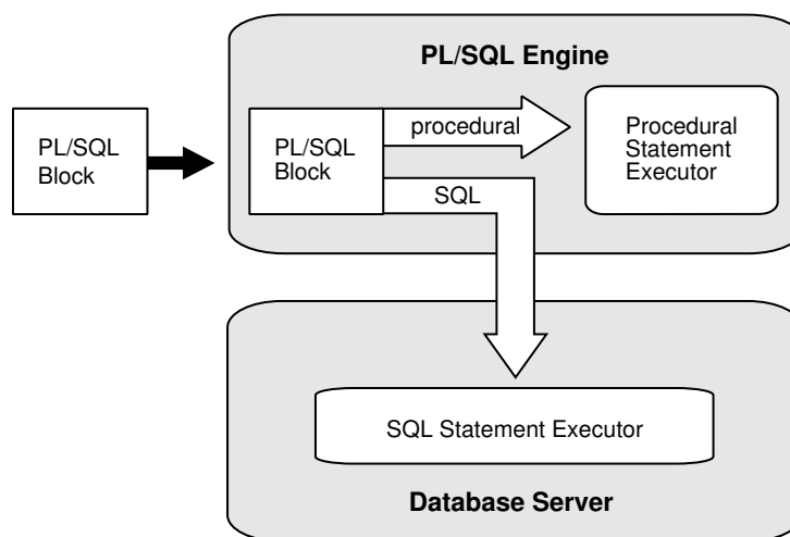
Figure 1-1 PL/SQL Engine
