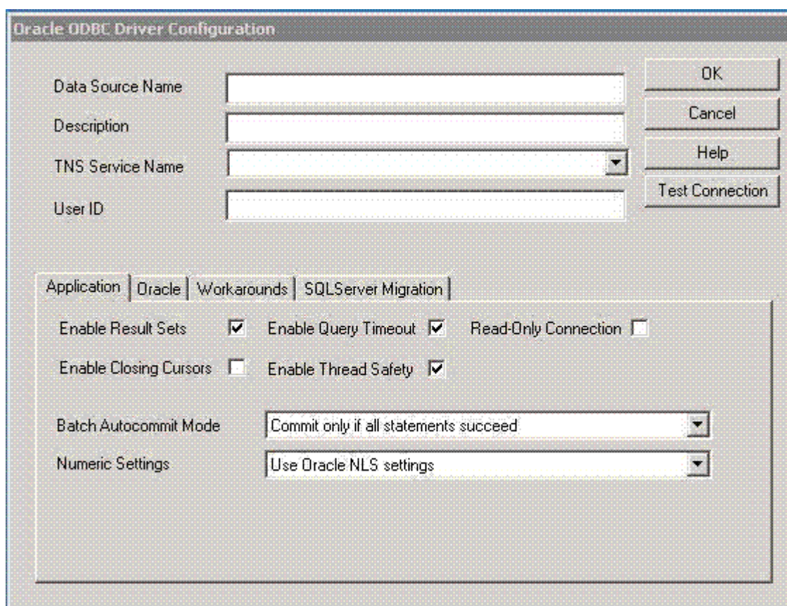
Figure 21–4 The Application Options Tab of the Oracle ODBC Driver Configuration Dialog Box
