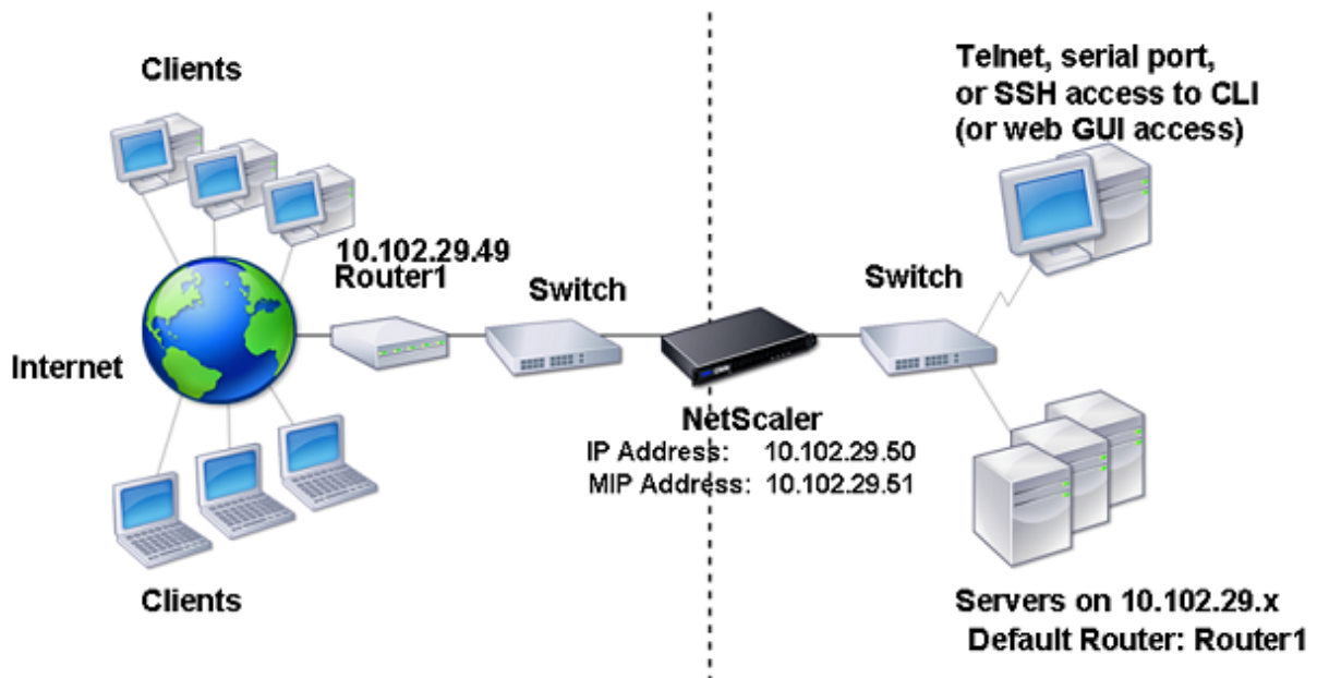
Figure 1. VLAN on a Single Subnet
