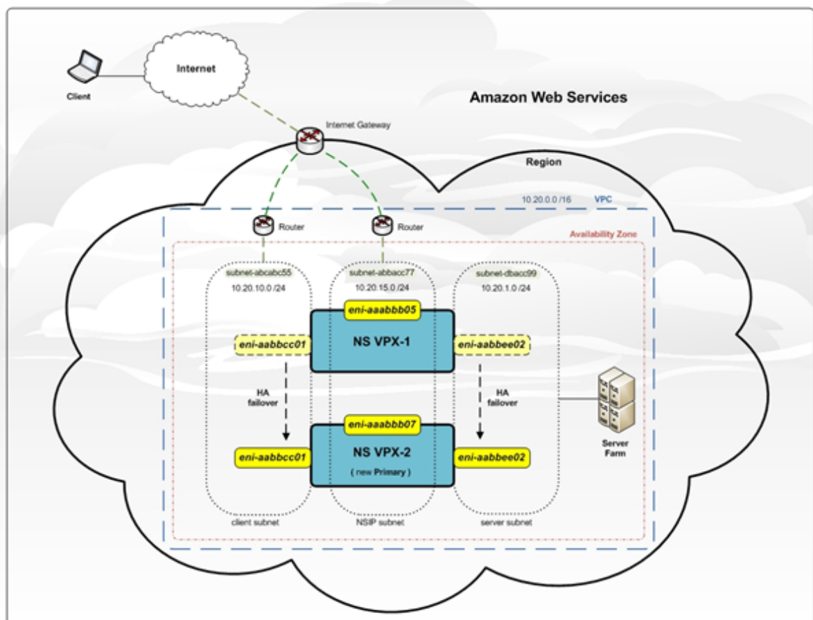
Figure 1. A Citrix ADC VPX HA Pair on AWS, using ENI migration
