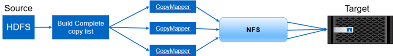
Hadoop DistCp and NetApp
