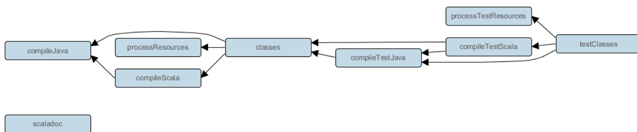
Figure 33. Scala plugin - tasks
