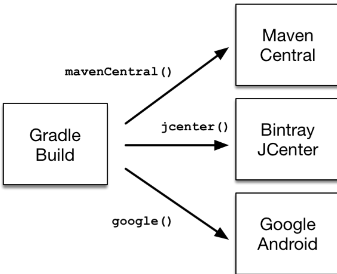
Figure 17. Declaring a repository with the help of shortcut methods
