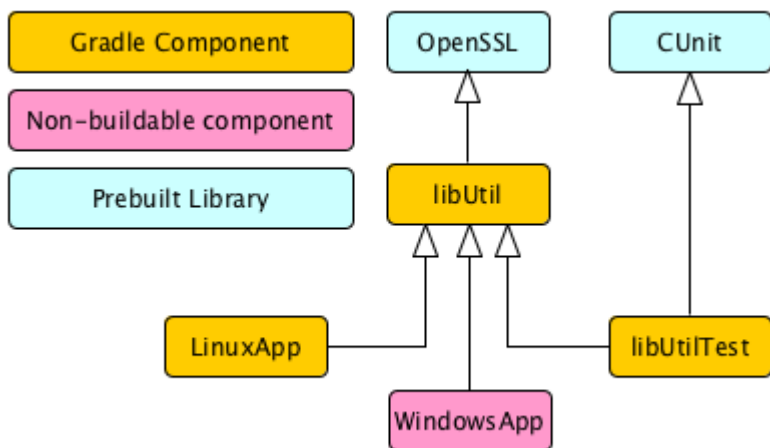
Figure 25. Dependent Components Example
