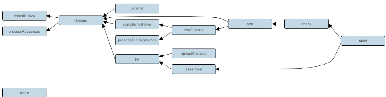
Figure 29. Java plugin - tasks
