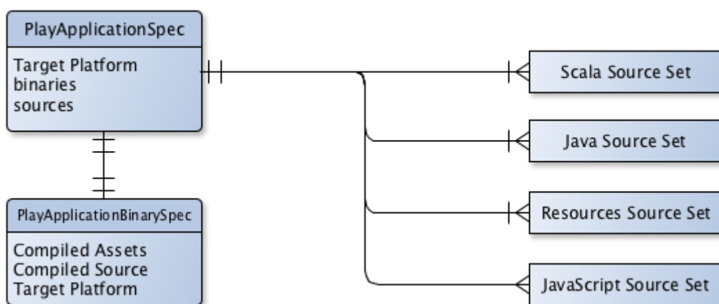
Figure 32. Play plugin - software model
