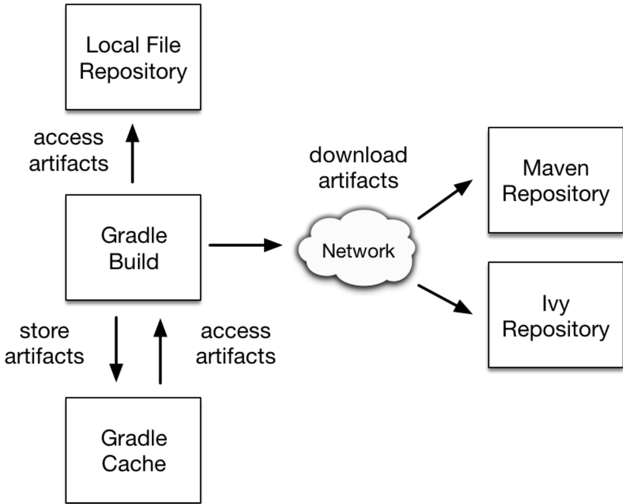
Figure 11. Dependency management big picture
