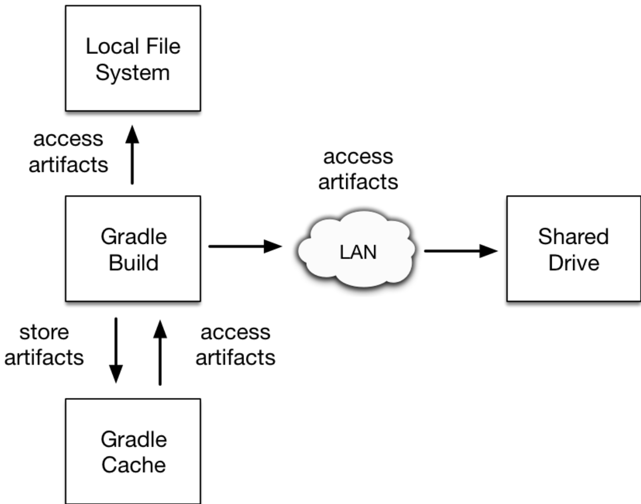
Figure 15. Resolving file dependencies from the local file system and a shared drive
