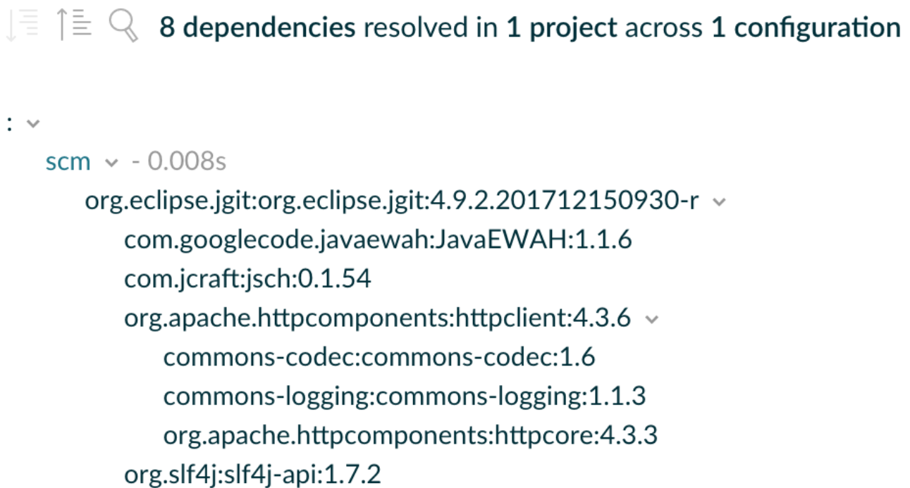
Figure 18. Dependency tree in a build scan
