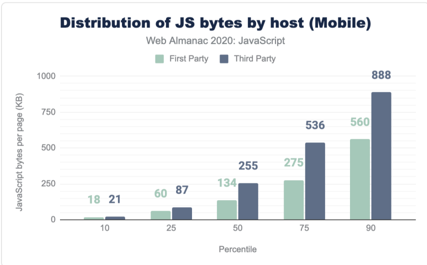
Figure 2.11. Distribution of the number of JavaScript bytes by host for mobile.
