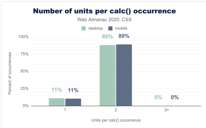
Figure 1.23. Distribution of the number of units per calc() occurrence.
