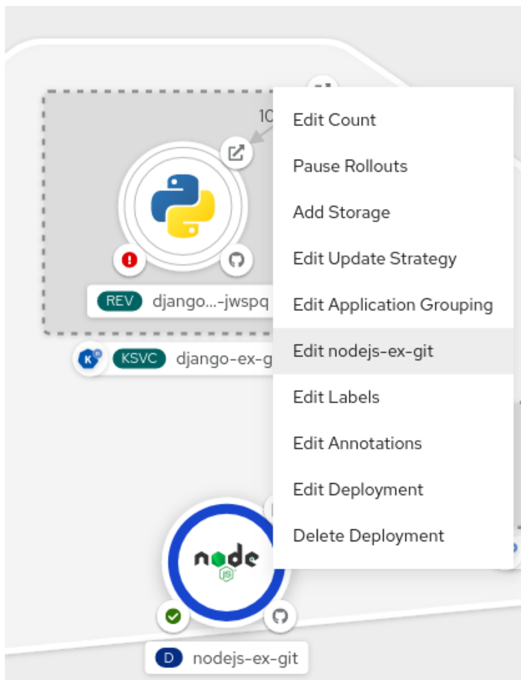
Figure 12.1. Edit application
