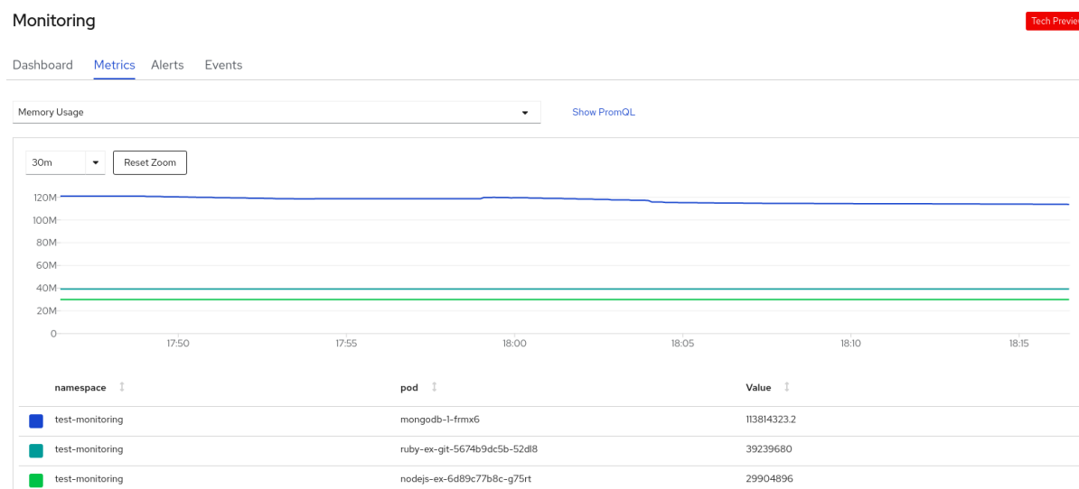
Figure 10.2. Monitoring metrics
