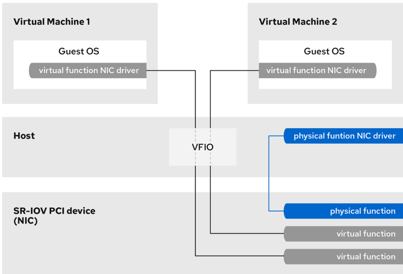
Figure 11.1. SR-IOV architecture
