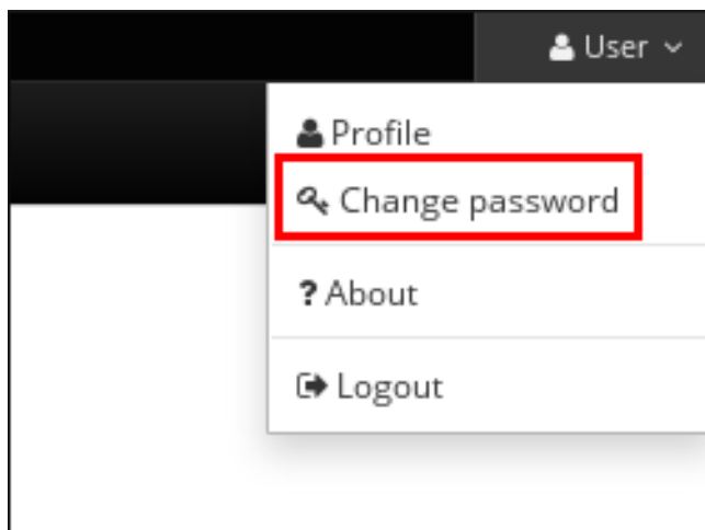
Figure 32.1. Resetting Password
