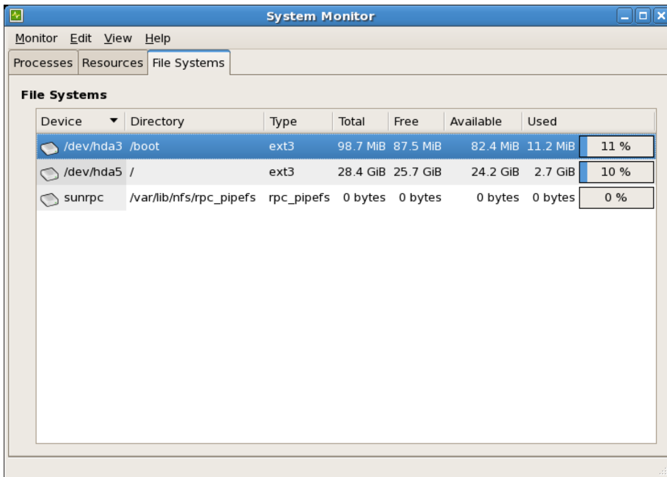
Figure 2.1. GNOME System Monitor File Systems tab
