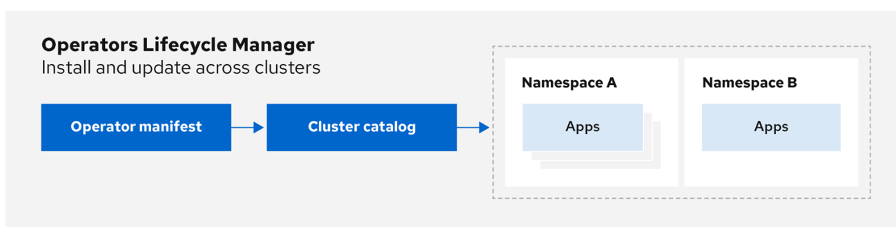
Figure 2.2. Operator Lifecycle Manager workflow
