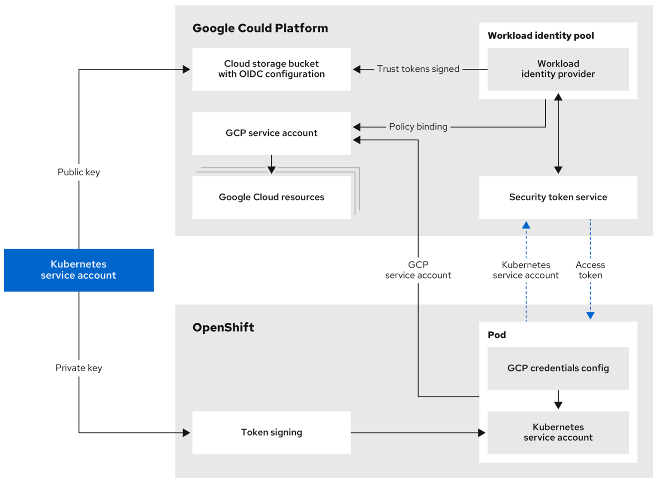
Figure 19.3. GCP Workload Identity authentication flow
