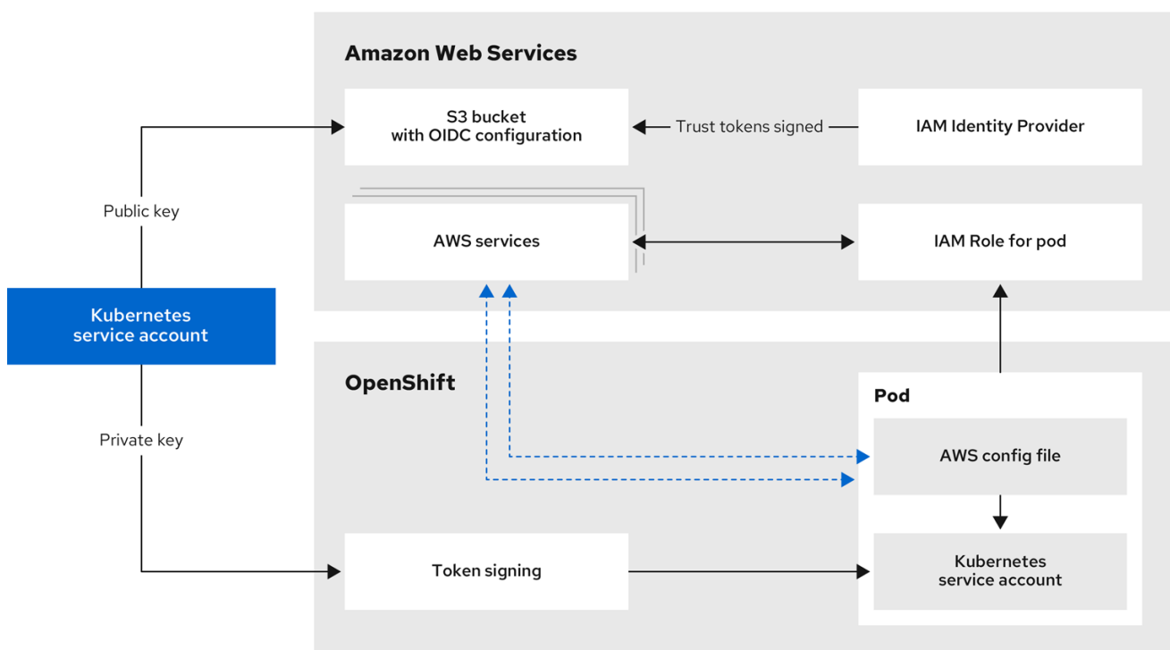
Figure 19.2. AWS Security Token Service authentication flow
