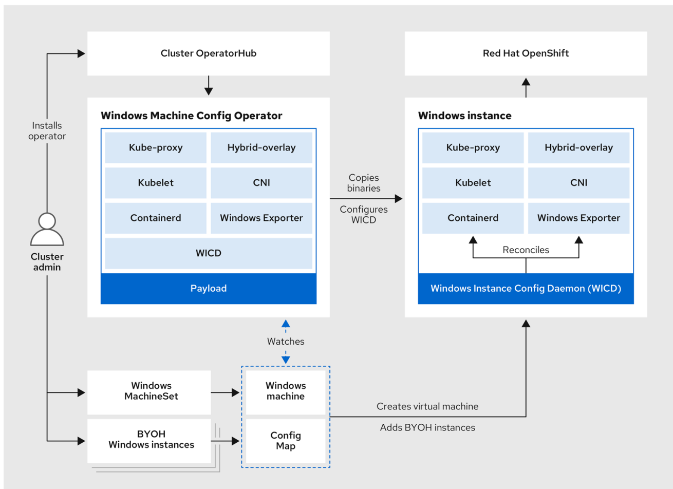
Figure 3.1. WMCO design
