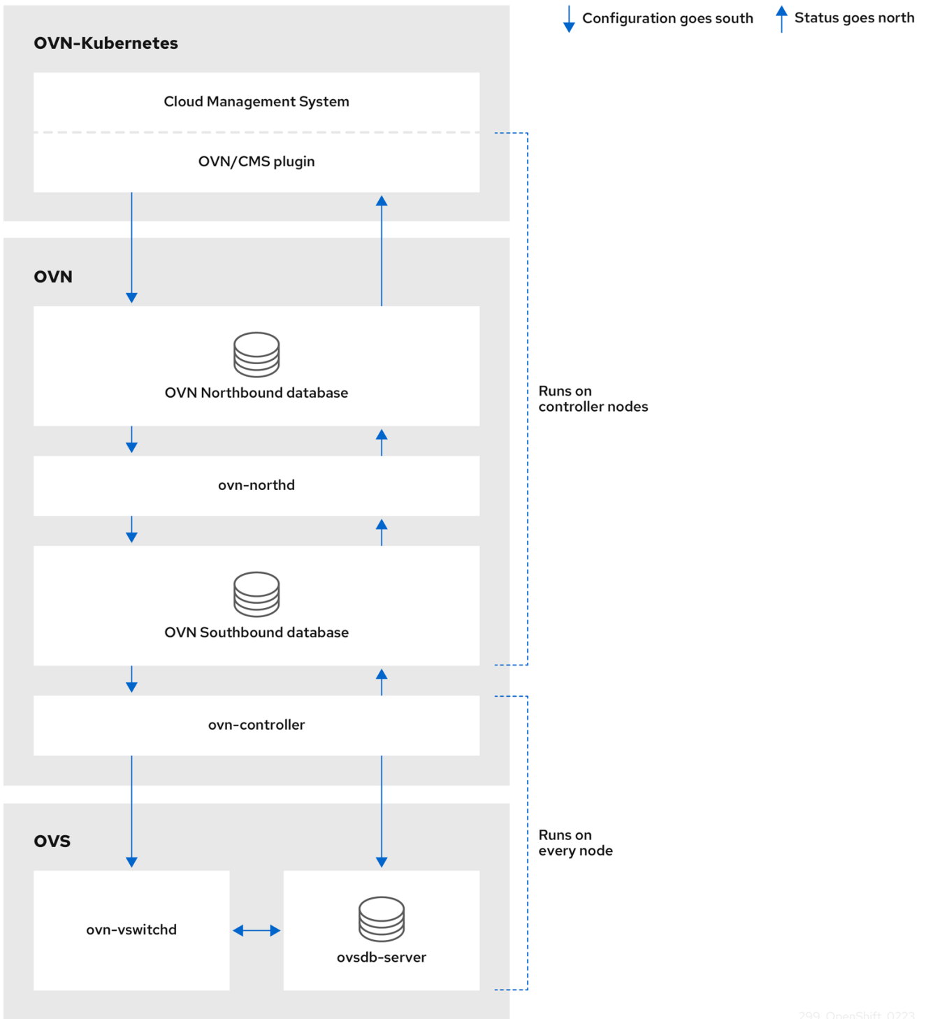
Figure 27.1. OVK-Kubernetes architecture
