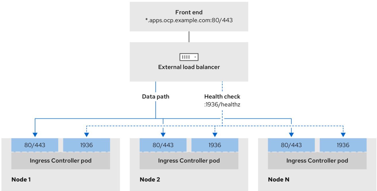
Figure 24.4. Example network workflow that shows an Ingress Controller operating in an OpenShift Container Platform environment
