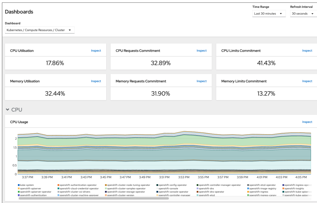
Figure 28.1. Example compute resources dashboard
