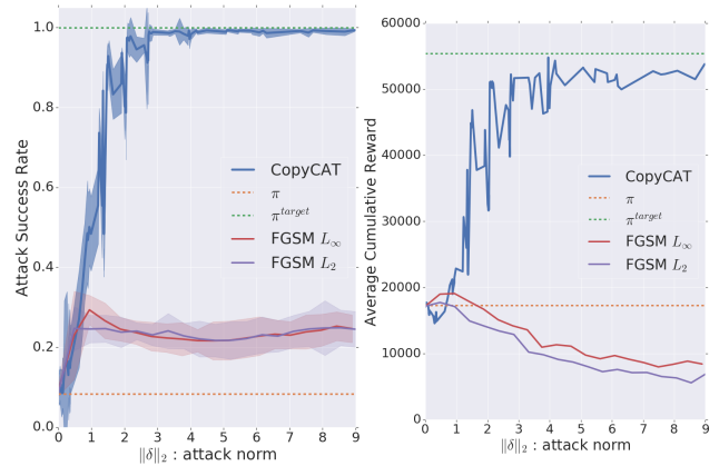
Figure 6: CopyCAT against FGSM for policy targeted attacks in HERO. On the left, the attack success rate. On the right, the average cumulative reward under attack.
