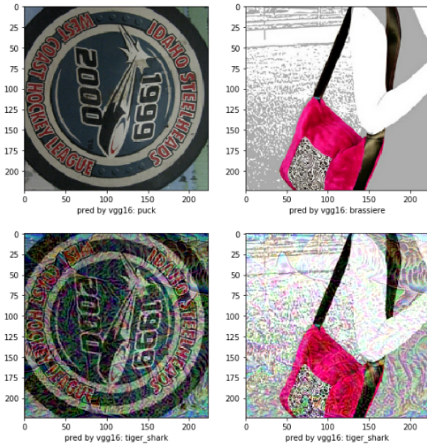
Figure 13: Top: images from the test set, unseen during the training of the attack. Down: attacked images: (image + attack). Below each image, the label predicted by VGG16.
