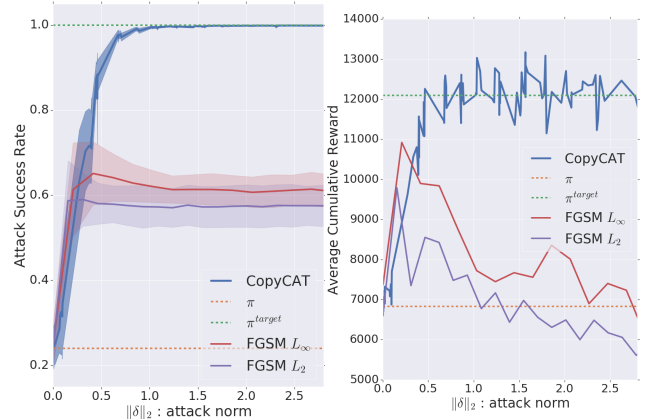
Figure 7: CopyCAT against FGSM for policy targeted attacks in Air Raid. On the left, the attack success rate. On the right, the average cumulative reward under attack.
