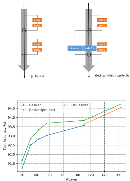
Figure 2. LM-architecture is an efficient structure that enables ResNet to achieve same level of accuracy with less parameters on CIFAR10.
