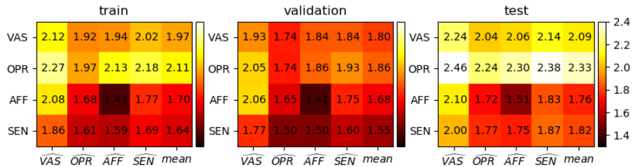
Figure 3: Average MAE matrices on training, validation and test data. The y-axis gives the true label, and the x-axis the prediction (or the mean of the 4 predictions). Each entry is the mean absolute difference between the two variables.
