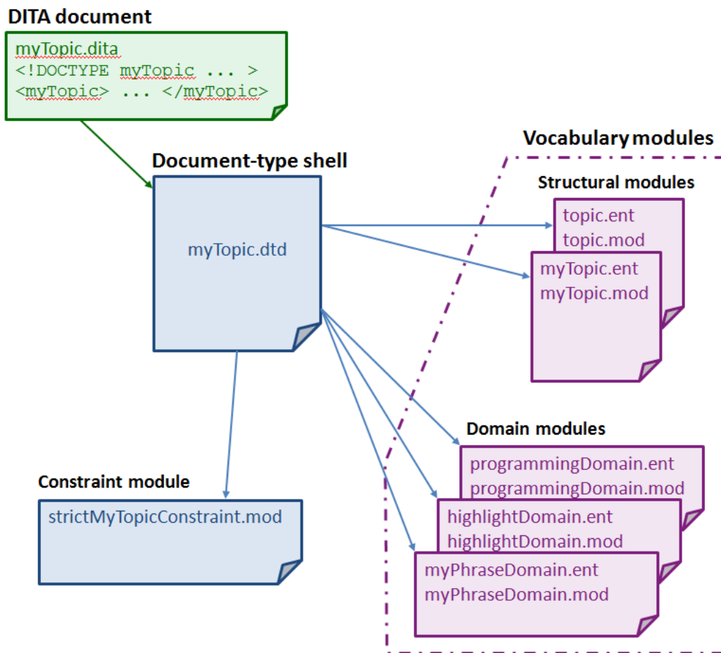
Figure 38: Document type shell
